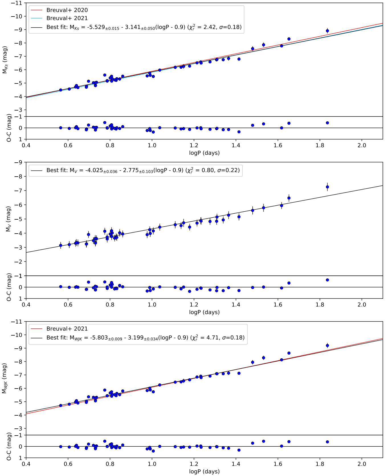
Fig. 5. Period-luminosity relations of Galactic Cepheids in K_S , V , and W_{JK} bands ( top , middle , and bottom , respectively) calibrated with Gaia EDR3 parallaxes (RUWE<1.4 only). The colored lines represent the relations from Breuval et al. (2020) and Breuval et al. (2021).
