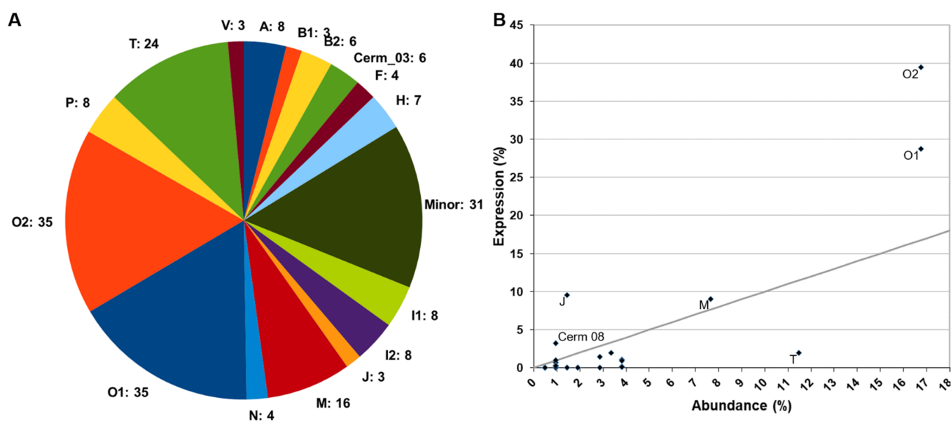
Figure 1. Summary of the diversity of conotoxins of Cylinderothamnium ammiralis based on the venom gland transcriptome. (A) Distribution in superfamilies of the 209 identified conotoxin precursors. The number beside the name represents the number of peptides within the superfamily. The minor superfamilies are expanded in Supplementary Materials Figure S1. (B) Scatter plot displaying the correlation between the number of peptides and the relative expression (measured in Transcripts Per Million, TPMs) for each superfamily. The two values were transformed to percentage. The gray line represents the 1:1 correlation between the two axes.
