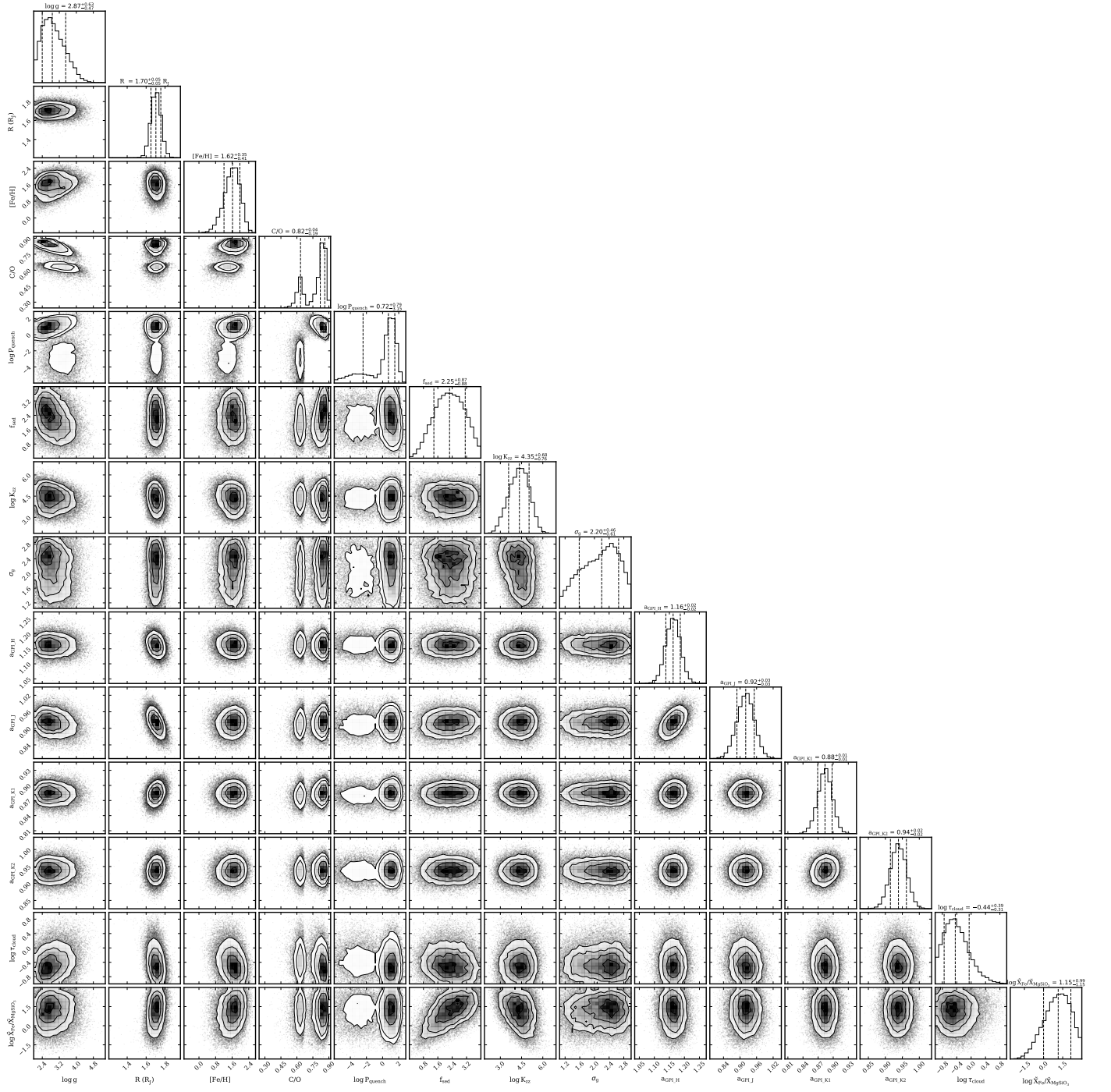
Fig. C.7. Posterior distribution of the spectral retrieval with petiRADTRANS.
