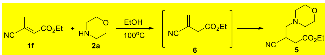
Scheme 4. Addition of morpholine to ethyl 3-cyanobut-2-enoate 1e .
