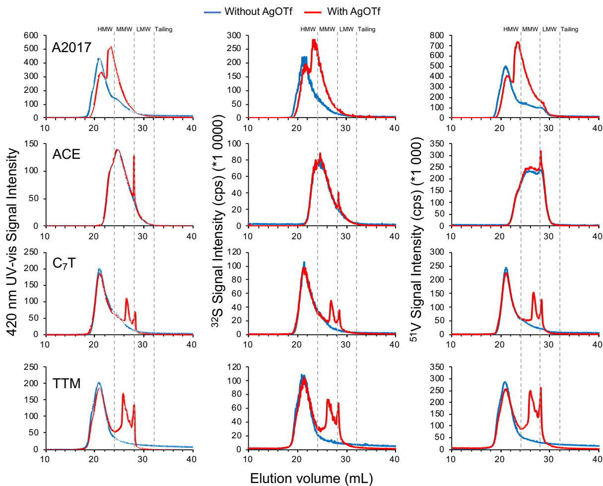
Figure 2. UV-vis absorption at 420 nm (left) and 32 S (middle) and 51 V (right) GPC ICP-HR-MS chromatograms of A2017, ACE, C7T and TTM with (red trace) and without (blue trace) the addition of AgOTf.
