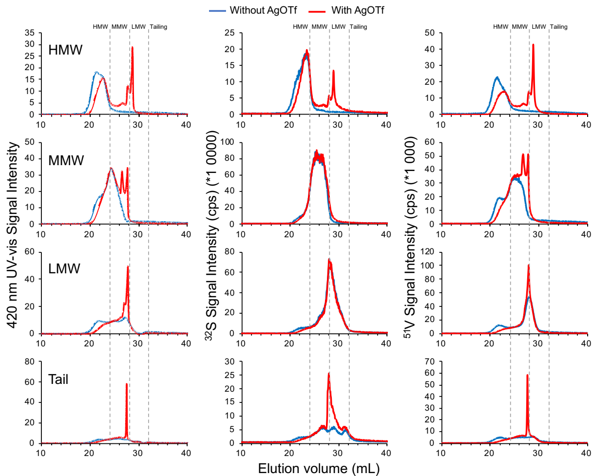
Figure 3. UV-vis absorption at 420 nm and ^{32}\text{S} and ^{51}\text{V} GPC ICP-HR-MS chromatograms of preparative GPC fractions of AR with and without the addition of AgOTf.
