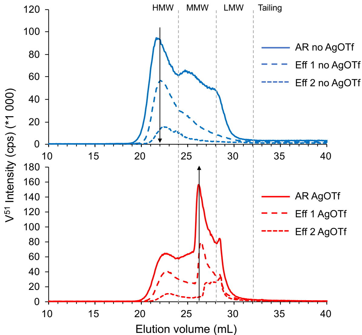
Figure 5. Graphs of AR, Eff 1, and Eff 2 with and without AgOTf for V (Ar, solid line; Eff 1, dashed line; and Eff 2, dotted line)
