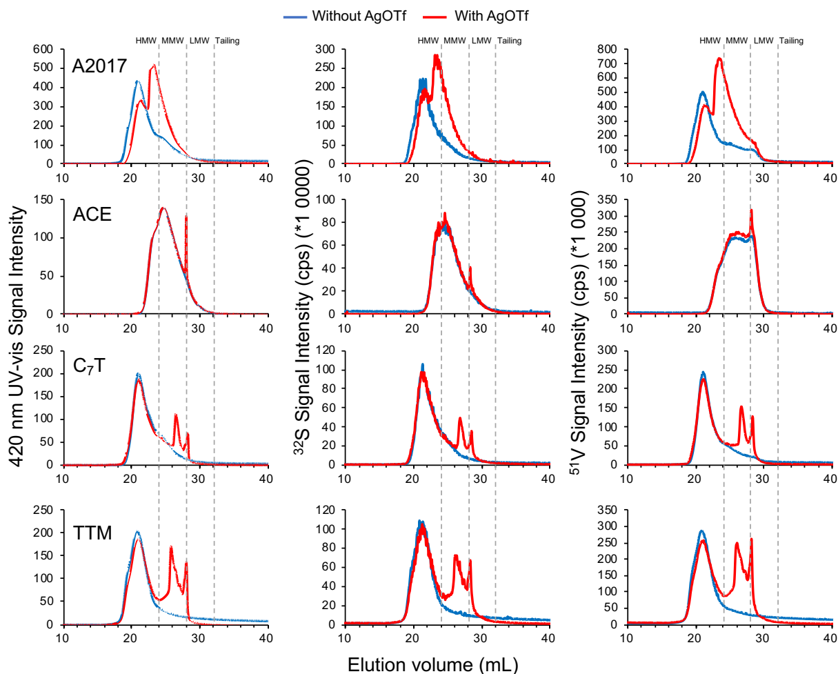
Figure 2. UV-vis absorption at 420 nm (left) and ^{32}\text{S} (middle) and ^{51}\text{V} (right) GPC ICP-HR-MS chromatograms of A2017, ACE, C7T and TTM with (red trace) and without (blue trace) the addition of AgOTf.
