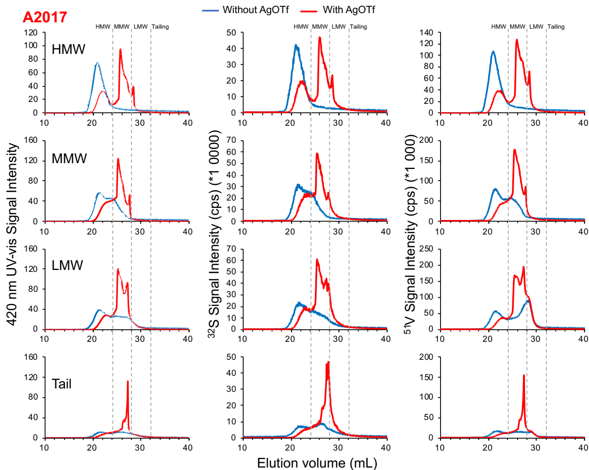
Figure 4. UV-vis absorption at 420 nm and ^{32}\text{S} and ^{51}\text{V} GPC ICP-HR-MS chromatograms of preparative GPC fractions of A2017 with and without the addition of AgOTf.
