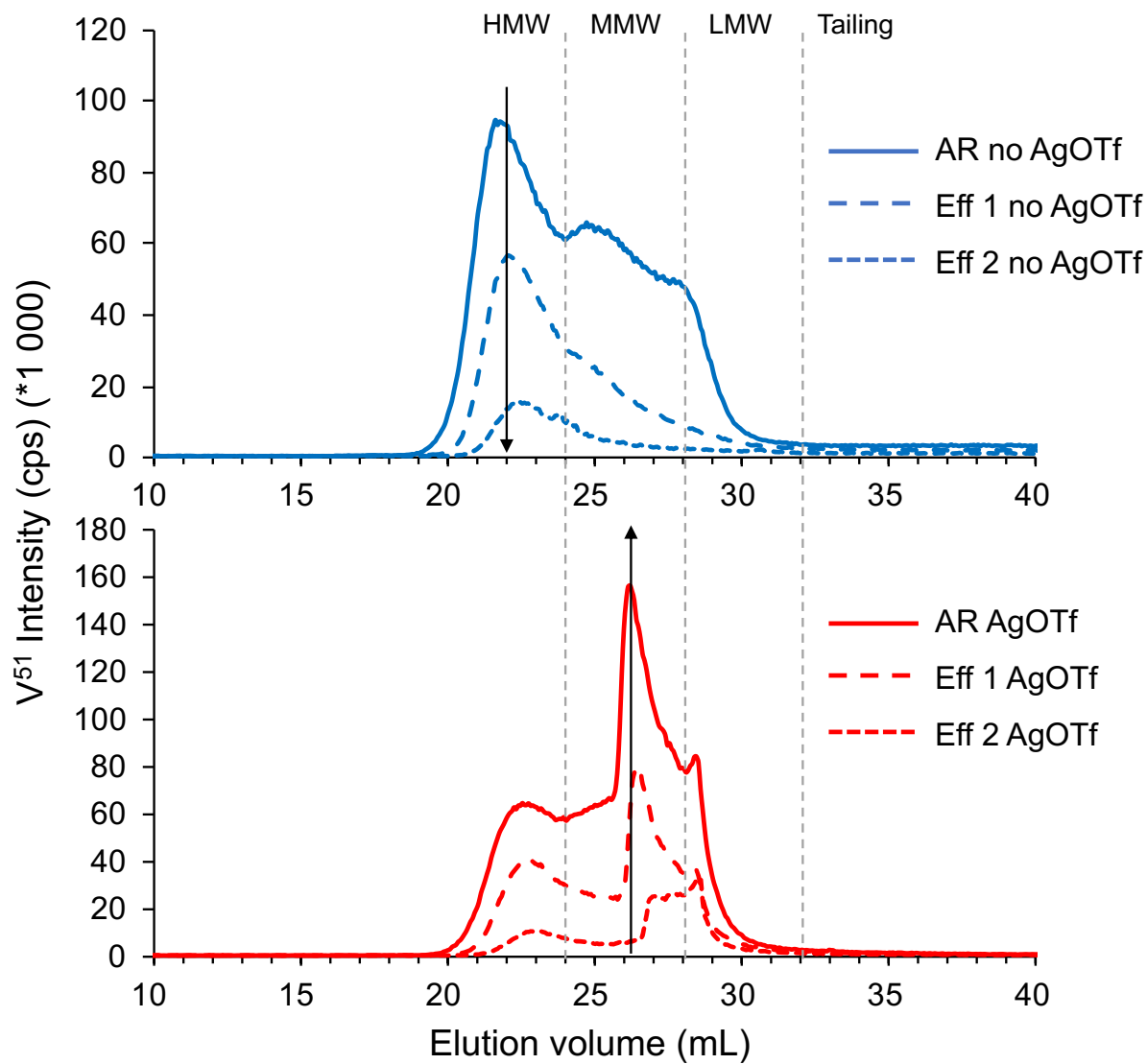
Figure 5. Graphs of AR, Eff 1, and Eff 2 with and without AgOTf for V (Ar, solid line; Eff 1, dashed line; and Eff 2, dotted line)
