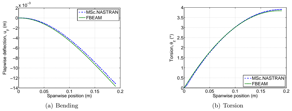
FIGURE 3 – FBEAM validation by MSc. NASTRAN
