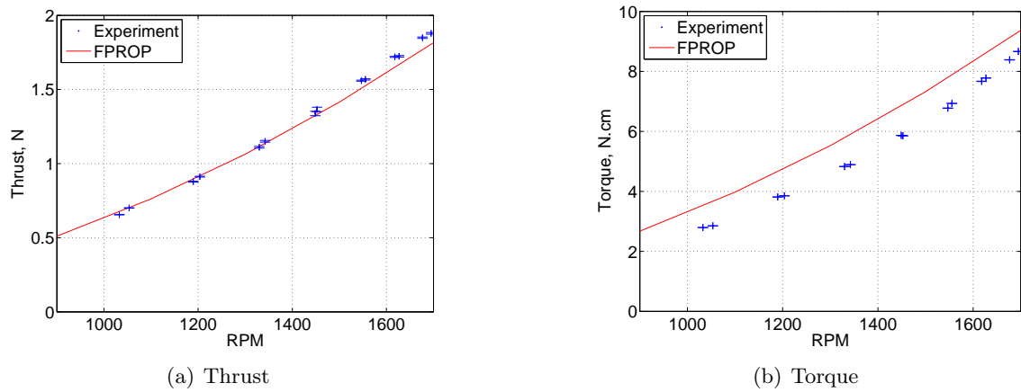
FIGURE 5 – Thrust and torque of rigid and flexible propotor at different rotational speed ( V=0 )
