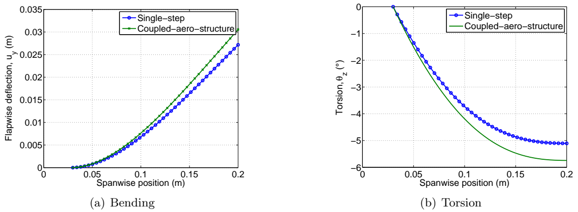
FIGURE 4 – The effect of SS and CAS simulation on the blade deformations
