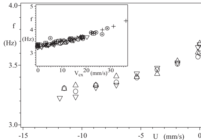
FIGURE 3 – Experimental variation of the transverse oscillation frequency as a function of the mean flow velocity U for free plexiglas cylinders of length L_c = 55 mm and of different ratios D/H = 0.46 ( \nabla ), D/H = 0.53 ( \circ ), D/H = 0.56 ( \triangle ). The flowing fluid is a water-glycerol solution ( C = 10\% ). Inset : variation of the oscillation frequency f as a function of V_{cx} for cylinders of diameter D = 1.5 mm ( D/H = 0.53 ) and of different lengths : L_c = 10 (+), 20 ( \otimes ), 30 ( \oplus ), 40 ( \boxplus ), 55 ( \circ ), 60 ( \square ), 70 ( \times ) and 80 mm (*). Data points corresponding to D = 1.3 mm ( \nabla ) and D = 1.6 mm ( \triangle ) with L_c = 55 mm have been added for comparison.
