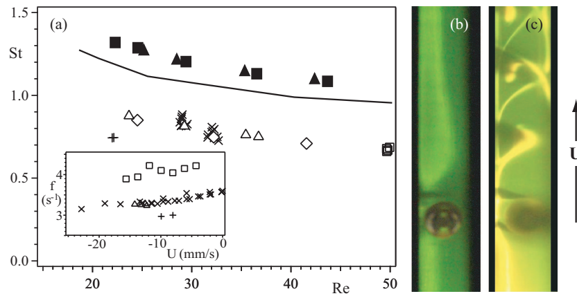
FIGURE 4 – a) Variations of the Strouhal number fH/V_r of the oscillations of plexiglas cylinders as a function of the Reynolds number Re for V_{cx} = 0 - Free cylinder ( L_c/W = 0.61 , D/H = 0.53 ) ( \diamond ) : water-glycerol solutions and ( \triangle ) : water-salt-glycerol solutions of concentrations 0, 5, 10 and 15 % (the data points are in this order from right to left). Tethered cylinder : D/H = 0.64 , L_c/W = 0.98 in water ( \blacksquare ) and in solution WN ( \blacktriangle ). Continuous line : numerical simulation. - Inset : variation with U of the frequency for water glycerol solutions of concentrations 0 % ( \square ), 10 % ( \times ), 20 % ( + ) (these data are also plotted on the main graph). b)-c) Visualizations from the side of the cell of fluorescent dye injected upstream of a tethered cylinder kept fixed (b) or free to oscillate (c). The cell is illuminated by a laser sheet parallel to the (x, y) plane in the middle of the cell width.
