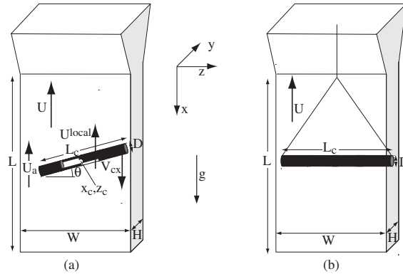
FIGURE 1 – Experimental setup. a) Free cylinder : U : mean flow velocity, V_{cx} : vertical component of the cylinder velocity. b) Tethered cylinder.
