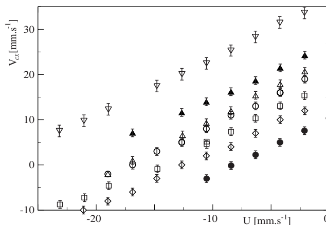
FIGURE 2 – Vertical velocity V_{cx} of free cylinders of diameter D in solutions WN1 or WN2 (see Tab. 1) as a function of the fluid velocity U . Open symbols : oscillating cylinders; solid symbols : no oscillations. plexiglas cylinders ( \rho_s = 1.20 \text{ g.cm}^{-3} ) - ( \triangle ), ( \blacktriangle ) : D = 1.5 \text{ mm} ( D/H = 0.53 ), WN1 ; ( \circ ), ( \bullet ) : D = 1.6 \text{ mm} ( D/H = 0.56 ), WN1 for ( \circ ) and WN2 for ( \bullet ); ( \square ) : D = 1.8 \text{ mm} ( D/H = 0.63 ), WN1 ; ( \diamond ) : D = 2.1 \text{ mm} ( D/H = 0.74 ), WN1 . Carbon cylinder ( \rho_s = 1.54 \text{ g.cm}^{-3} ) - ( \nabla ) : D = 1.5 \text{ mm} ( D/H = 0.53 ), WN2 .
