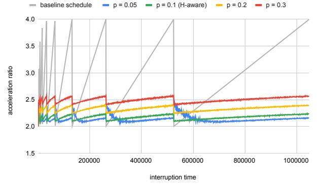
Figure 2: Acceleration ratios of Robust_p , for H = 0.1 .
