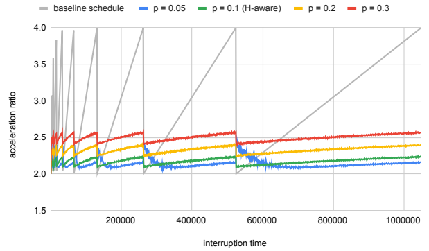
Figure 2: Acceleration ratios of Robust_p , for H = 0.1 .
