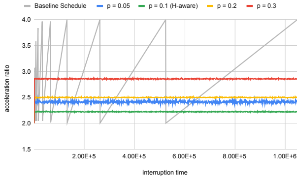
Figure 1: Acceleration ratios of X_{\tau(1-p)}^* , for H = 0.1 .
