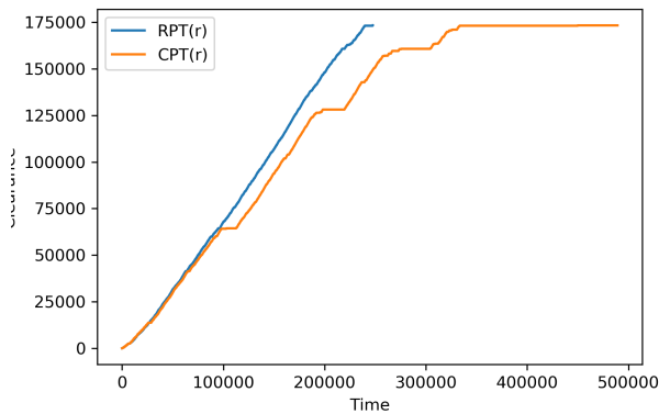
Figure 4: Comparison of the two strategies on the Berlin network (633 nodes, 1042 edges).
