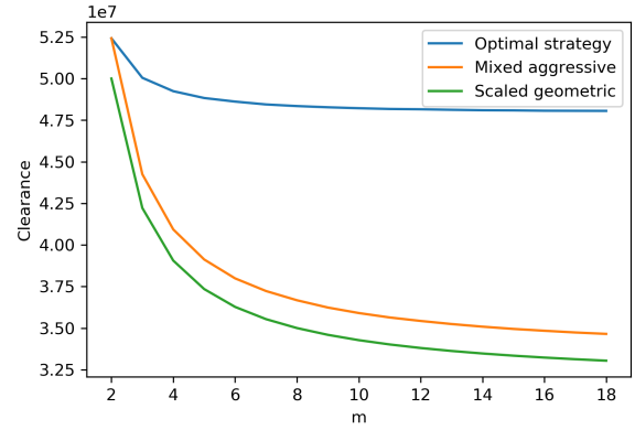
Figure 2: Clearance as function of m , for T = 10^8 and R = R_m^* .
