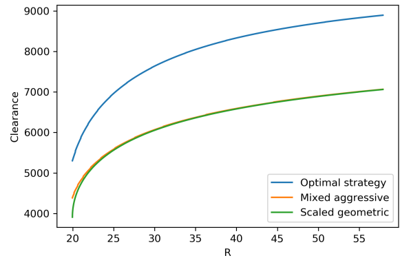
Figure 3: Clearance as function of R , for m = 4 and T = 10^4 .
