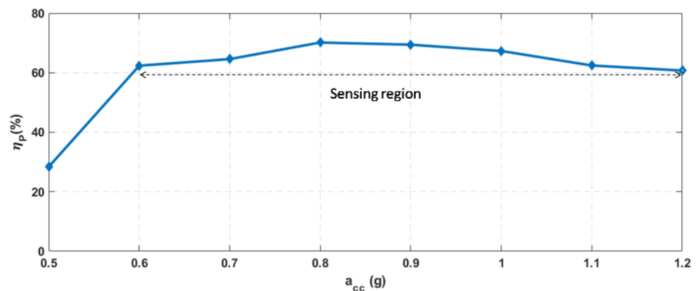
Figure 5. EAWVS power conversion efficiency \eta_p vs. acceleration a_{cc} (experimental results).
