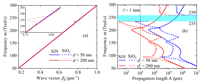
FIG. 2: Frequency spectra of the (a) wave vector and (b) propagation length of SPhPs propagating along nanofilms of SiN and SiO 2 of two thicknesses.
