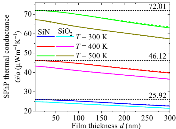
FIG. 4: SPhP thermal conductance per unit width of 1 mm-long nanofilms of SiN and SiO 2 , as a function of their thickness. The solid and dashed lines represent the respective analytical (Eq. (6)) and numerical [26] predictions, while the dotted ones stand for the quantum of thermal conductance predicted by Eq. (10). Calculations were done for three temperatures.
