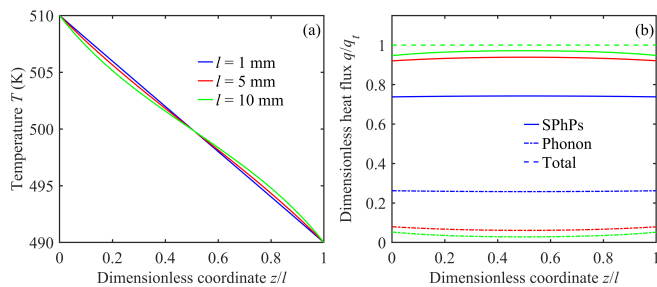
FIG. 3: Numerical results for the (a) temperature profile and (b) heat fluxes in a 50 nm-thick SiN film at 500 K. Calculations were done for three film lengths of practical interest.
