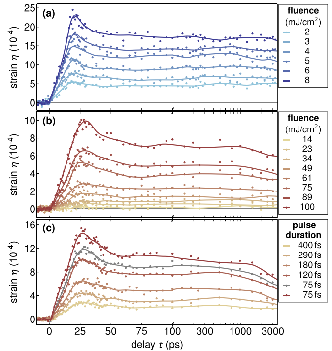
FIG. 2. Transient lattice strain \eta for different excitation parameters, measured with UXRD. Solid lines act as a guide to the eye. (a) Fluence series for \text{Bi}_2\text{Y}_1\text{Fe}_5\text{O}_{12} with femtosecond NUV excitation. For \text{Bi}_1\text{Y}_2\text{Fe}_5\text{O}_{12} we show (b) the fluence series with 120 \text{ fs} NIR excitation and (c) the pulse duration series with 100 \text{ mJ}/\text{cm}^2 NIR excitation. The gray data set has a similar pulse duration but opposite linear chirp.
