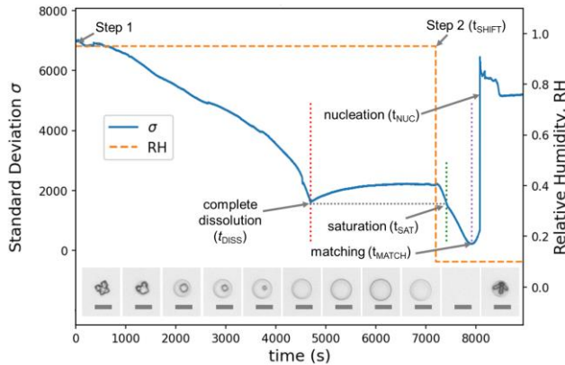
Figure 2. Typical (\sigma,t) -curve, during a full \%RH cycle (deliquescence/recrystallization), associated to each Region-Of-Interest (ROI). An illustrative ROI is provided in the lower part of the graph to show typical evolution of \mu D s. Characteristic time points are reported on both \%RH curve and (\sigma,t) -curve. \%RH cycle (dotted orange) goes from step 1 (crystal deliquescence up to t_{DISS} followed by \mu D dilution) to step 2 ( \mu D contraction) at time t_{SHIFT} . During contraction, \mu D is at saturation at time t_{SAT} , optically disappear at time t_{MATCH} , and crystals nucleate at time t_{NUC} .
