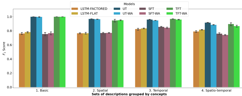
Figure 3: F1 scores for all the models on randomly held-out sentences. F_1 is measured on separated sets representing each category of concepts defined in Section 2.2.
