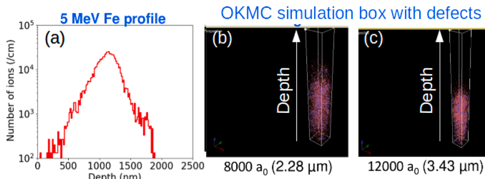
Fig. 8. (a) Depth profile of implanted 5 MeV Fe in Fe as obtained by Marlowe. Mega-OKMC simulation cell with a depth of (b) 2.28 μm and (c) 3.43 μm showing the location of the damage produced by the irradiation.
