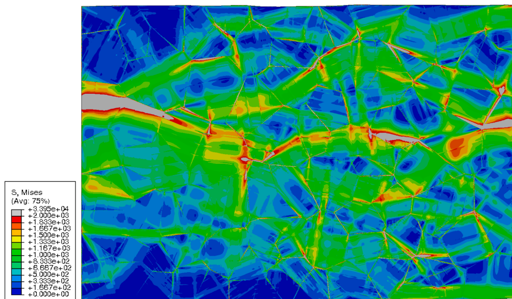
Fig. 30. Mises stress [MPa] field of an aggregate containing 110 grains, with four channels per grain, stretched in the horizontal direction to \langle \epsilon_{11} \rangle = 0.01 [1]. One slip system activated in between the channels, one slip system activated in the slip channels.
