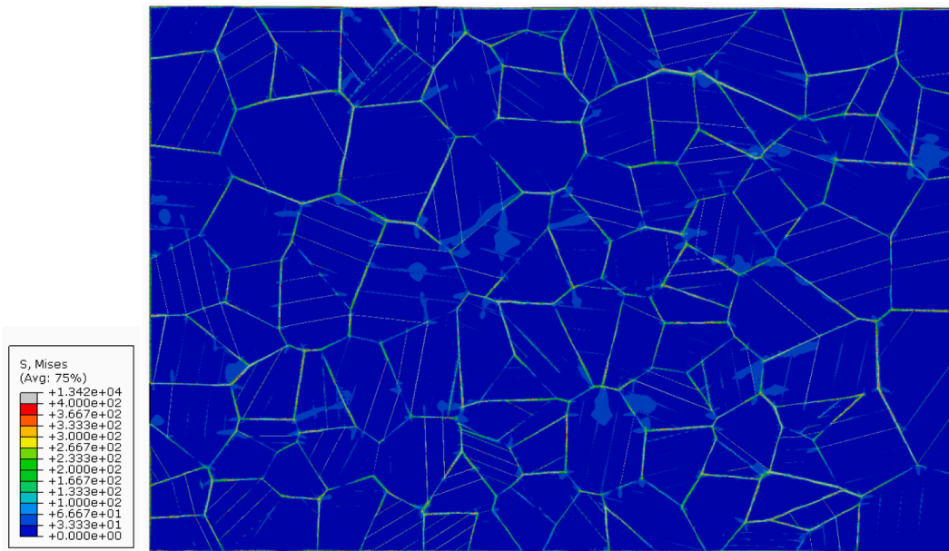
Fig. 29. Mises stress [MPa] field of an aggregate containing 110 grains, with four channels per grain, stretched in the horizontal direction to \langle \epsilon_{11} \rangle = 0.01 [ / ]. Three slip systems activated in between the channels, one slip system activated in the slip channels. Channels are clearly visible.
