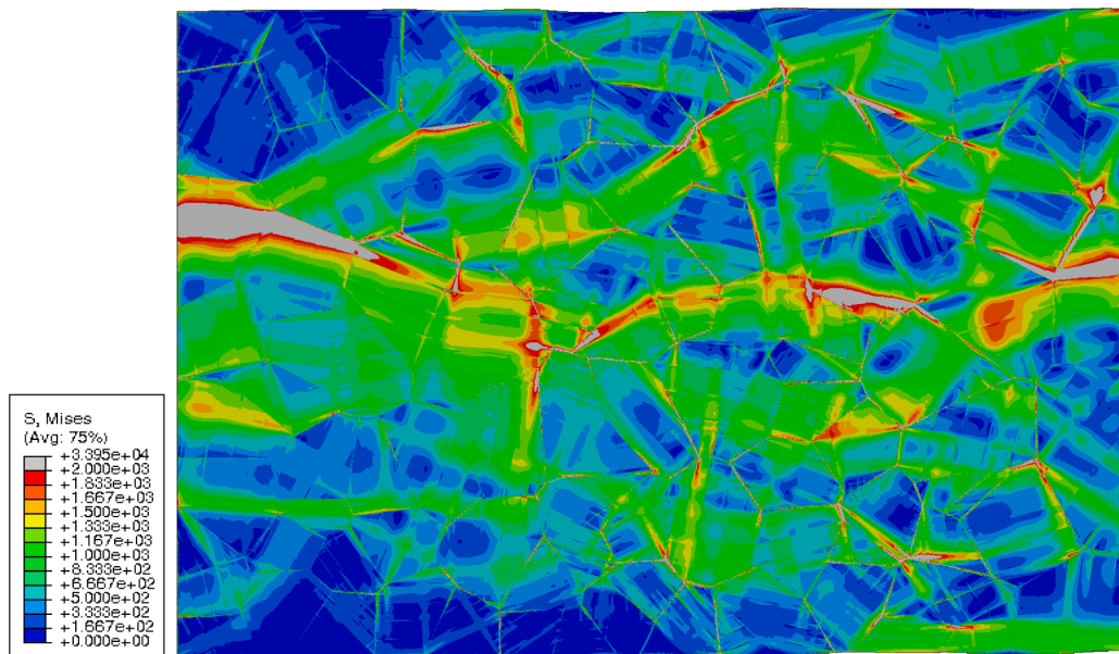
Fig. 30. Mises stress [MPa] field of an aggregate containing 110 grains, with four channels per grain, stretched in the horizontal direction to \langle \epsilon_{11} \rangle = 0.01 [ / ]. One slip system activated in between the channels, one slip system activated in the slip channels.
