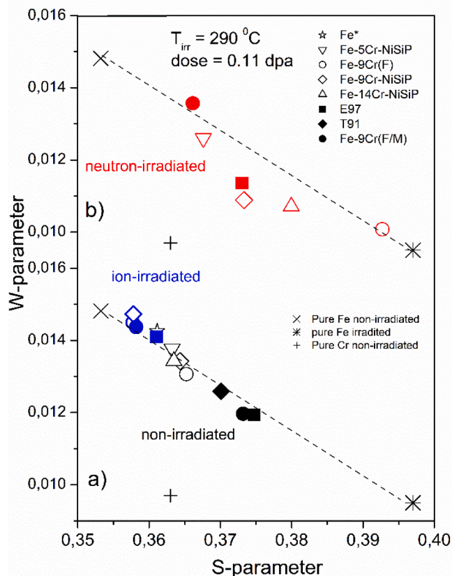
Fig. 10. S versus W parameters of a) ion irradiated and b) neutron irradiated FeCr alloys and steels considered in M4F. The results are compared with existing data of similar materials and steels.
