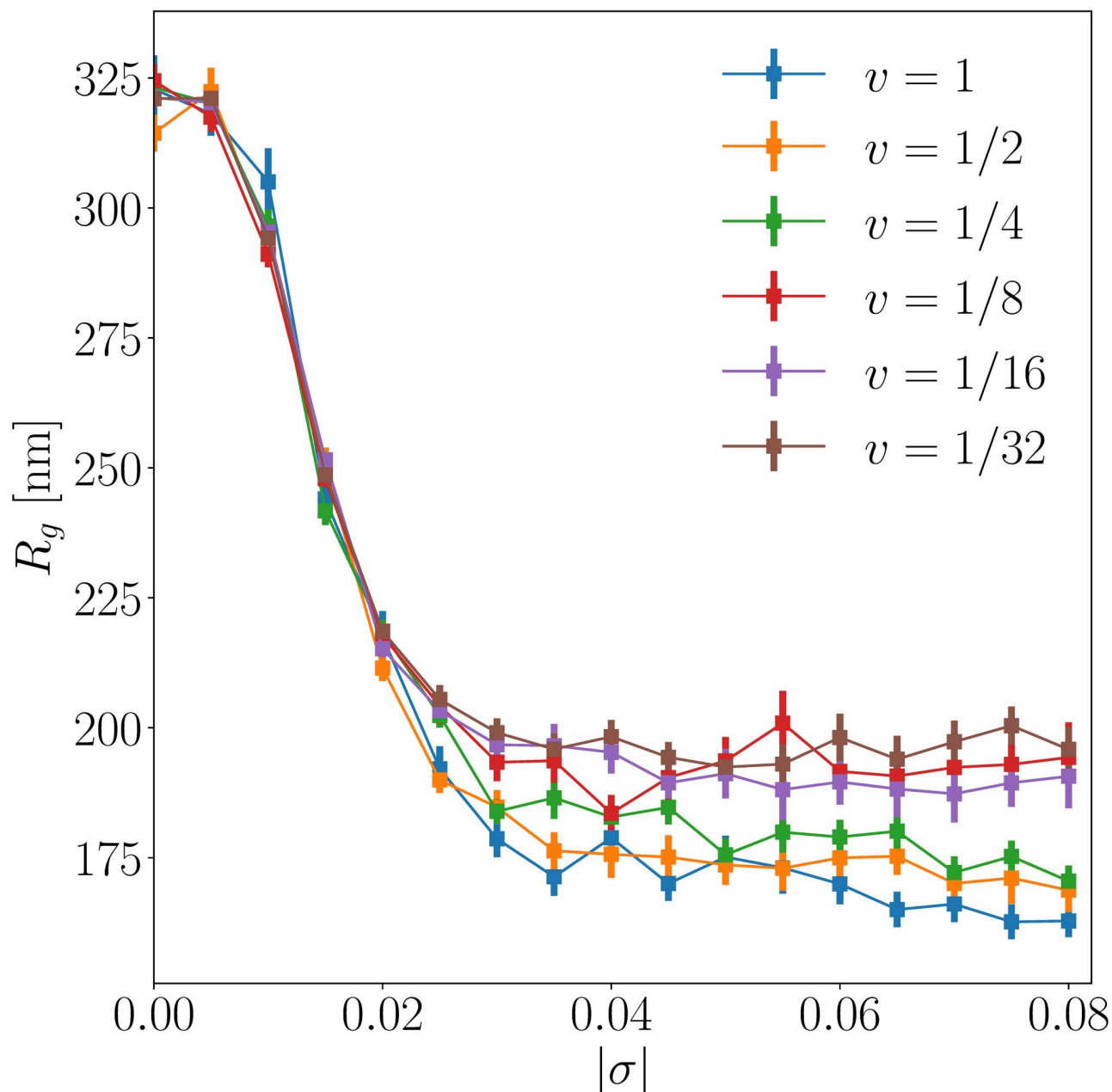
Fig 5. Sensitivity of results with respect to supercoiling variation rates. In this plot, a point corresponds to the mean value of the radius of gyration obtained at a given \sigma for a specific supercoiling rate v (see explanations for the protocol). The error bars correspond to the standard error of the mean computed over 20 different simulation runs.
