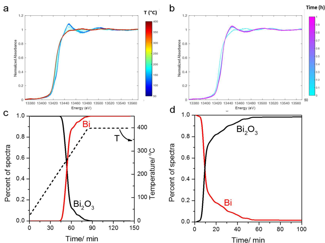
Figure 10. X-ray absorption spectra at the L 3 -absorption edge for bismuth phase evolution over CoBi/CNT catalyst, (a) reduction from 50 °C to 400 °C under H 2 . (b) reduced CoBi/CNT was contacted with air at 50 °C, (c) Bismuth speciation determined by MCR-ALS from the Quick-XAS data set recorded for the CoBi/CNT catalyst during (c) H 2 activation and (d) air passivation.
