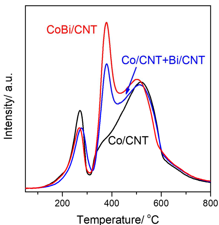
Figure 2. TPR profiles of the freshly calcined CNT-supported cobalt catalysts.
