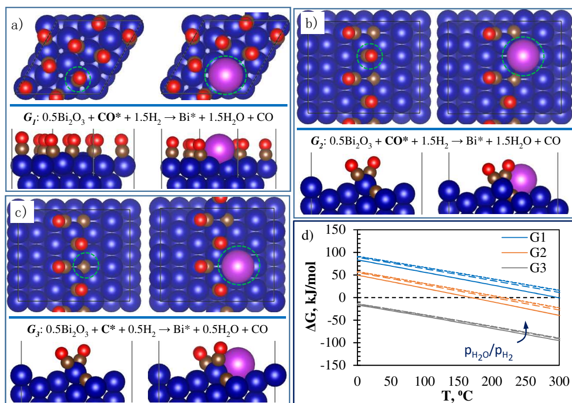
Figure 13. Thermodynamic analysis of the competitive adsorption between (a) Bi and CO* on Co(111) terraces, (b) Bi and CO* at (211) step sites and (c) Bi and C* at Co(211) step sites. (d) Reaction Gibbs free energy for the displacement of CO* and C* by Bi at FT conditions (6.7 bar CO, 13 bar H 2 , and H 2 /H 2 O ratio of 1 – 10.7). More details can be found in Figure S15, SI .
