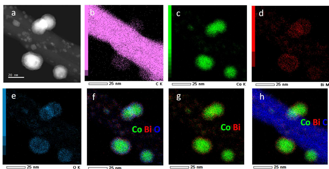
Figure 4. STEM-HAADF micrograph (a) and STEM-EDX elemental maps (b-f) of the activated CoBi/CNT catalyst (2wt.% Bi): (b) chemical map of C, (c) chemical
