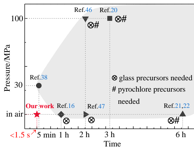
Figure 8. Pressure demand versus consolidating time during the synthesis of (\text{La},\text{Y})_2(\text{Zr},\text{Ti})_2\text{O}_7 pyrochlore-based glass-ceramics at the cooling rate of 500\text{ }^\circ\text{C/s} via melting method together with some typical sintering and crystallization methods of the preparation of pyrochlore-based glass-ceramics waste form.
