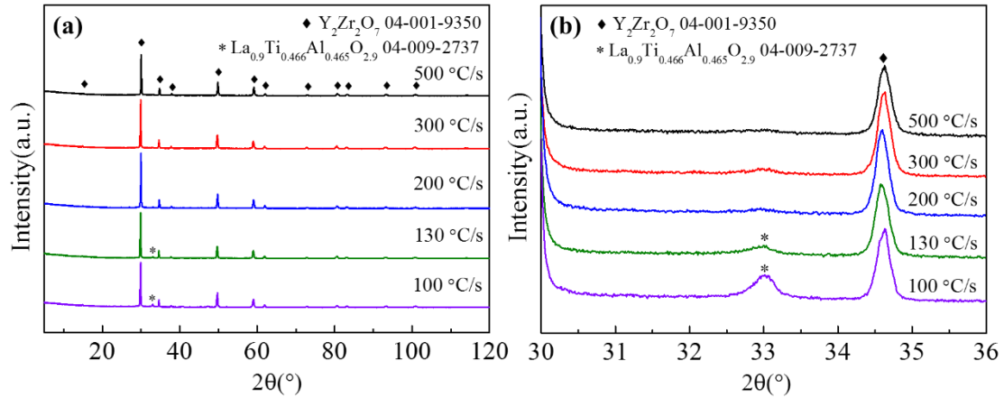
Figure 3. XRPD patterns of the as-synthesized (\text{La},\text{Y})_2(\text{Zr},\text{Ti})_2\text{O}_7 pyrochlore-based glass-ceramics at different cooling rates (a) and the enlargement of XRPD patterns in 30^\circ\sim 36^\circ revealing the secondary crystallization evolution (b). The average cooling rates were 100^\circ\text{C/s} , 130^\circ\text{C/s} , 200^\circ\text{C/s} , 300^\circ\text{C/s} and 500^\circ\text{C/s} (free cooling), respectively.
