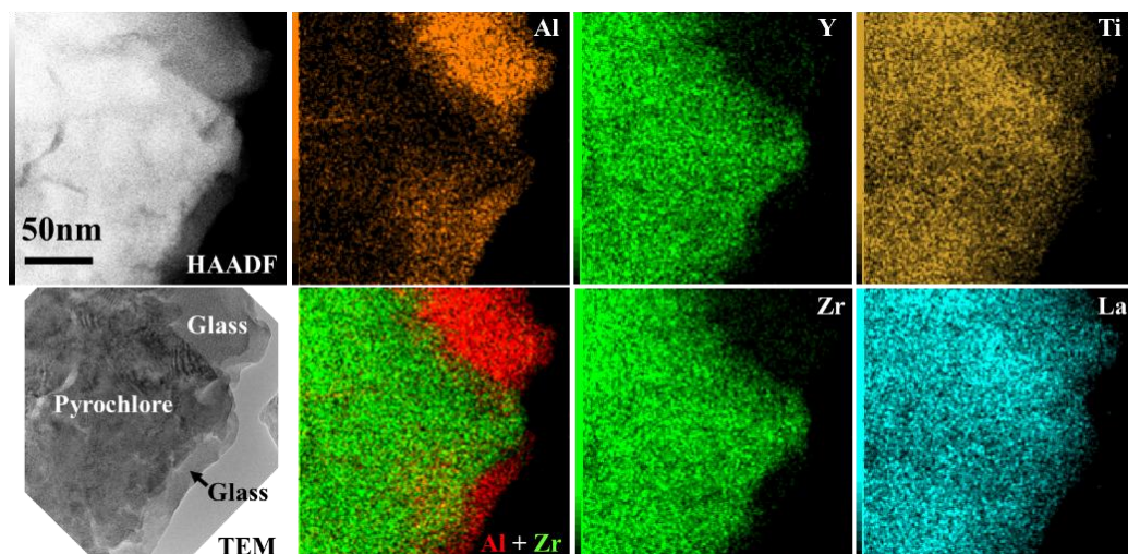
Figure 6. STEM-HAADF image and corresponding STEM-EDS cationic elemental maps of the as-synthesized (La,Y)_2(Zr,Ti)_2O_7 pyrochlore-based glass-ceramics at the cooling rate of 500 °C/s. The corresponding TEM image and the overlaid EDS maps of Al (glass) and Zr (pyrochlore).
