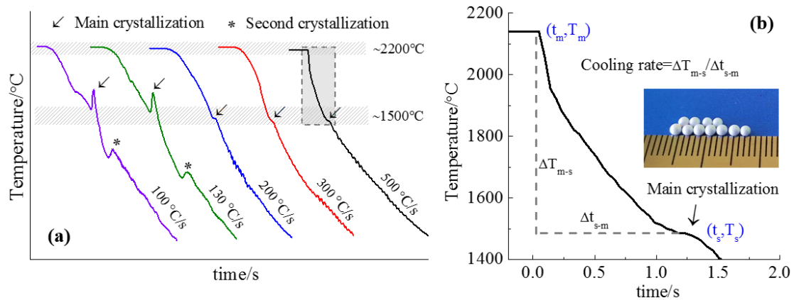
Figure 2. Cooling curves of samples during melt solidification. (a) Temperature-time profiles of
