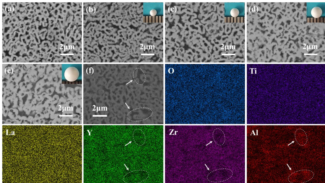
Figure 4. SEM images and corresponding EDS elemental maps of the as-synthesized (La,Y)_2(Zr,Ti)_2O_7 pyrochlore-based glass-ceramics. (a) Back scattering images of the polished sample with a cooling rate of 500 °C/s. (b-e) Back scattering images of the polished sample with a cooling rate of 500 °C/s.
