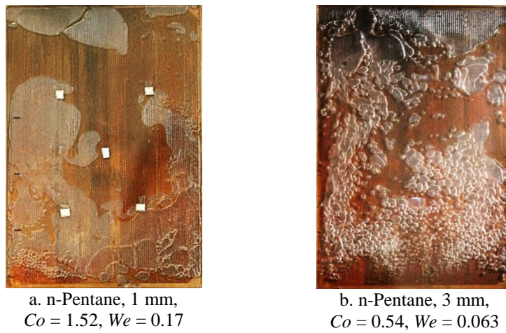
Figure 13: Effect of the confinement on the flow patterns of n-pentane for a high fill charge. Q = 100\text{ W} , FR = 150\% , T_{sink} = 10^{\circ}C .
