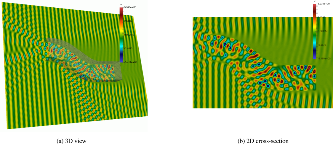
Figure 3: The COBRA cavity problem.
