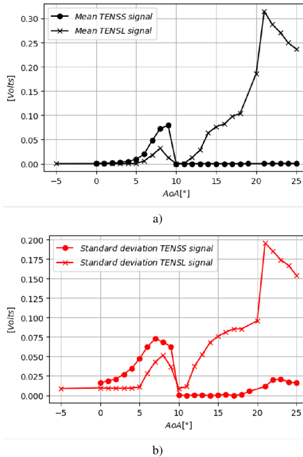
Figure 11. Comparison of the mean a) and the standard deviation b) of the signal of the TENSLS (reference case) and TENSSE e-Telltale as function of AoA
