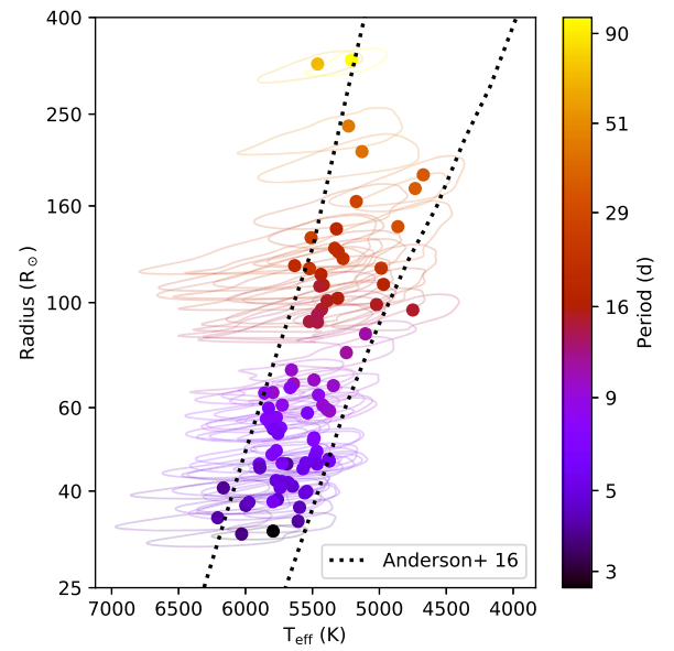
Figure 3. Radius versus temperature diagram for the Galactic Cepheids. The dots are the average values (over the pulsation), whereas the thin lines show the values over the pulsation. The color code refers to the pulsation period. The dotted lines are the borders of the theoretical instability strip, using mild rotation (0.5) and solar metallicity (Anderson et al. 2016). We only use the Cepheids with period greater than 12 days for building our template light curves; see Section 4.3.1 for further details.
