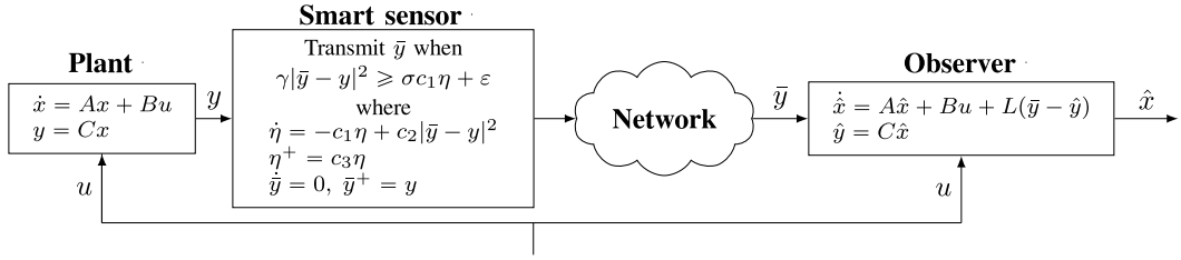
Fig. 1. Block diagram representing the system architecture
