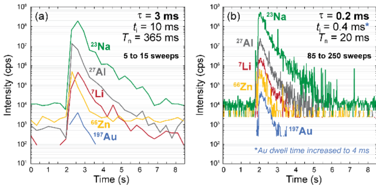
Figure 1. Transient time-resolved LA-ICP-MS signals of two single shot analyses (60 \mu\text{m} laser spot) in NIST SRM610 glass using two different timing setups: (a) long and (b) short settling ( \tau ), dwell ( t_i ) and sweep ( T_n ) times. Intensities for a total of 28 analytes were acquired in both cases (amu 7, 11, 23, 25, 27, 29, 34, 35, 39, 43, 55, 57, 63, 66, 75, 79, 85, 88, 95, 107, 121, 133, 137, 140, 197, 208, 209, 238), only 5 are shown.
