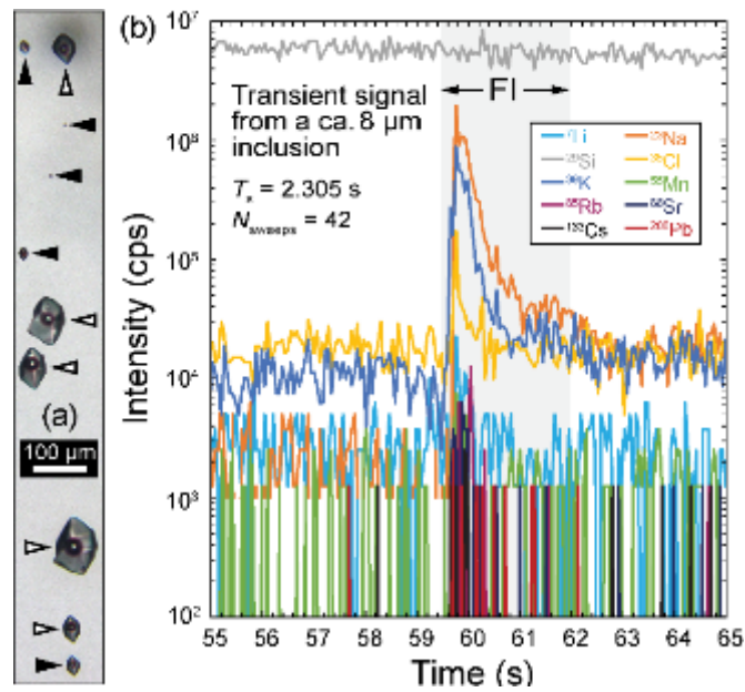
Figure 2. (a) Microphotograph showing representative aqueous, liquid (L) + vapor (V) inclusions in quartz sample KMP-1; empty arrows show the typical size of inclusions previously analyzed by LA-ICP-MS ( \geq 20 \mu\text{m} ) 18 ; filled arrows show the typical size of inclusions targeted here ( \leq 20 \mu\text{m} , down to 4 \mu\text{m} ). (b) Transient time-resolved LA-ICP-MS signals from a fluid inclusion ca. 8 \mu\text{m} in diameter in sample KMP-1, showing intensities for 10 out of 52 measured elements; T_s corresponds to the total transient signal duration.
