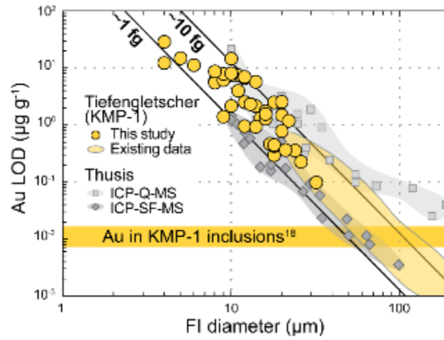
Figure 4. Limits of detection (LOD) for Au as a function of approximate fluid inclusion (FI) diameter in sample KMP-1, compared to existing data on the same fluid inclusion assemblage 18 and from inclusions of similar type in the same context (aqueous fluids with ca. 4 wt.% NaCl in quartz from an Alpine fissure vein near Thusis, Switzerland) measured with two different ICP-MS systems 12 . The solid black lines indicate absolute Au LODs of ca. 1 and 10 fg.
