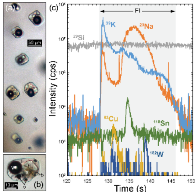
Figure 5. (a) Photomicrograph showing representative polyphase brine inclusions from sample Loww9. (b) Detail of one inclusion showing the nature of internal phases: aqueous liquid (L), vapor bubble (V), halite (h), another chloride salt (s) and unidentified opaque (o) or birefringent (b) crystals. (c) Transient time-resolved LA-ICP-MS signal from a brine inclusion ca. 60 \mu\text{m} in diameter in sample Loww9, showing intensities for 6 out of 52 measured elements; note the short, sharp peaks displayed by the metals (Cu, Sn, W) compared to the K and Na signals recording aqueous liquid and/or salt crystals.
