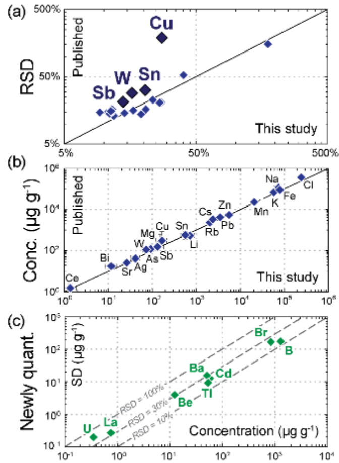
Figure 6. Quantitative results from the analysis of brine inclusions in sample Loww9. (a) Comparison of the relative standard deviation (RSD) of element concentrations in fluid inclusions analysed in this study compared with published data 19 ; note the improvement for Cu, Sn, Sb and W due to more representative recording of very short signals resulting from the ablation of tiny, metal-rich daughter phases. (b) Comparison of average element concentrations (Conc.) obtained in the fluid inclusions analysed in this study compared with published data 19 . (c) Plot of standard deviation (SD) vs. average concentration for 8 elements newly quantified (quant.) in this study, which were not included in the element list in previous work owing to scanning time constraints.
