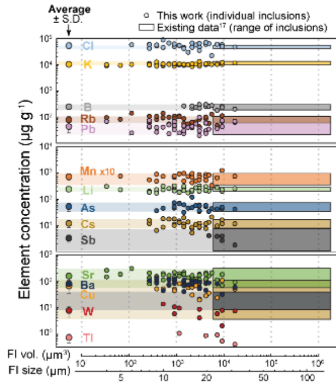
Figure 3. Concentrations obtained for 15 elements in fluid inclusions from sample KMP-1, as a function of fluid inclusion (FI) volume (vol.) and size. The dots correspond to analyses obtained here, and the coloured boxes depict the size and compositional range of inclusions analysed in a previous study using a conventional quadrupole 18 . Larger dots with error bars correspond to the average \pm standard deviation of analyses obtained in this study.
