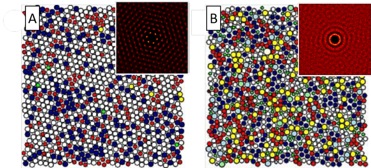
Figure 6. Snapshots of the final configuration of particle assemblies obtained by 2D Monte Carlo simulations for two polydispersities (A) 6 %, (B) 15 %. The different colors correspond to various particle sizes. The inserts show the two-dimensional pair distribution functions for the given particle assemblies.
