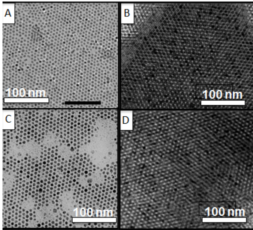
Figure 9 : TEM images of a monolayer (A) and a multilayer (B) of solution-phase annealed 7.1 nm hcp-Co single-crystals. TEM images of a monolayer (C) and a multilayer (D) of 7.0 nm hcp-Co single-crystals, obtained by dry-annealing of a native monolayer and multilayer of fcc-Co polycrystals.
