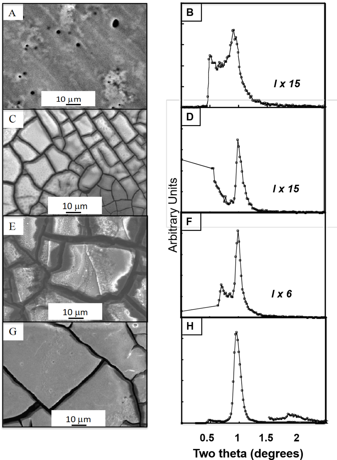
Figure 11 : SEM images obtained by depositing of cobalt nanoparticles on HOPG substrate at various temperatures: (A) 10 °C, (C) 25 °C, (E) 35 °C, (G) 45 °C. B, D, F and H, corresponding diffractograms.
