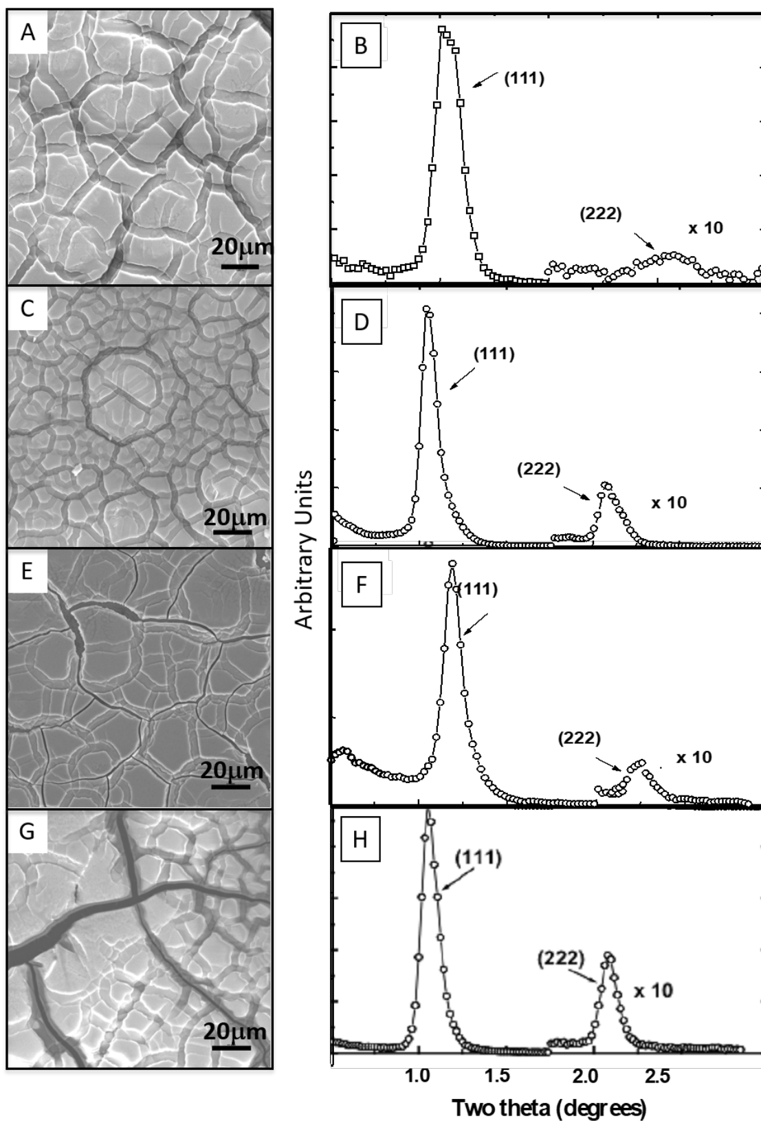
Figure 15 : SEM images of a supercrystalline film (thinner region) of 7.5 nm Co nanoparticles not annealed (A), annealed at 250 °C (C), at 300 °C (E) and at 350 °C (G). B, D, F and H, corresponding diffractograms.
