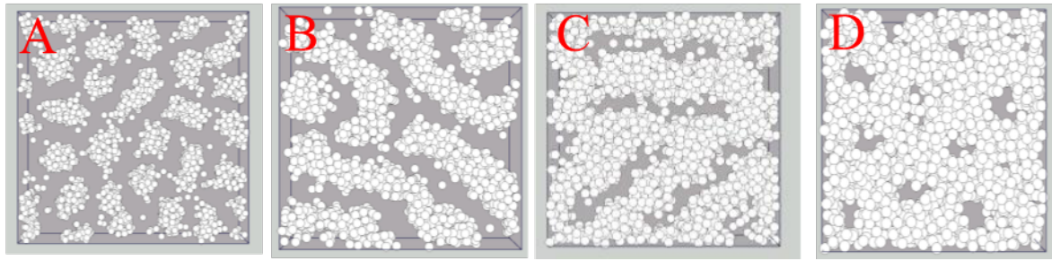
Figure 18. Snapshots of configurations for a confined Stockmayer fluid at \mu=2.0 , T=1.25 , L=10 and H=30 . A) \rho=0.1 , B) \rho=0.3 , C) \rho=0.4 , D) \rho=0.5 .
