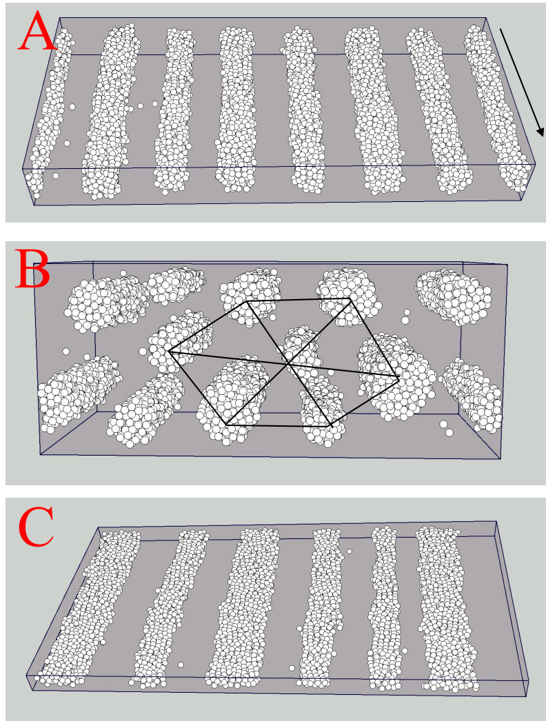
Figure 17. Snapshots of configurations for a confined Stockmayer fluid at \mu=2.0 , \rho=0.2 , T=1.25 , and H=20 . A) L=10 , B) L=27 , C) L=4 .
