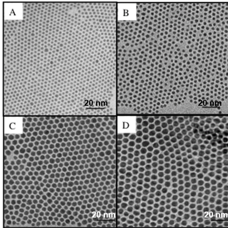
Figure 8 : TEM images of 2D ordered arrays of native fcc-Co polycrystals (a) 3.9 nm (S1), (b) 4.6 nm (S2), (c) 7.7 nm (S6), (d) 9.3 nm (S7).
