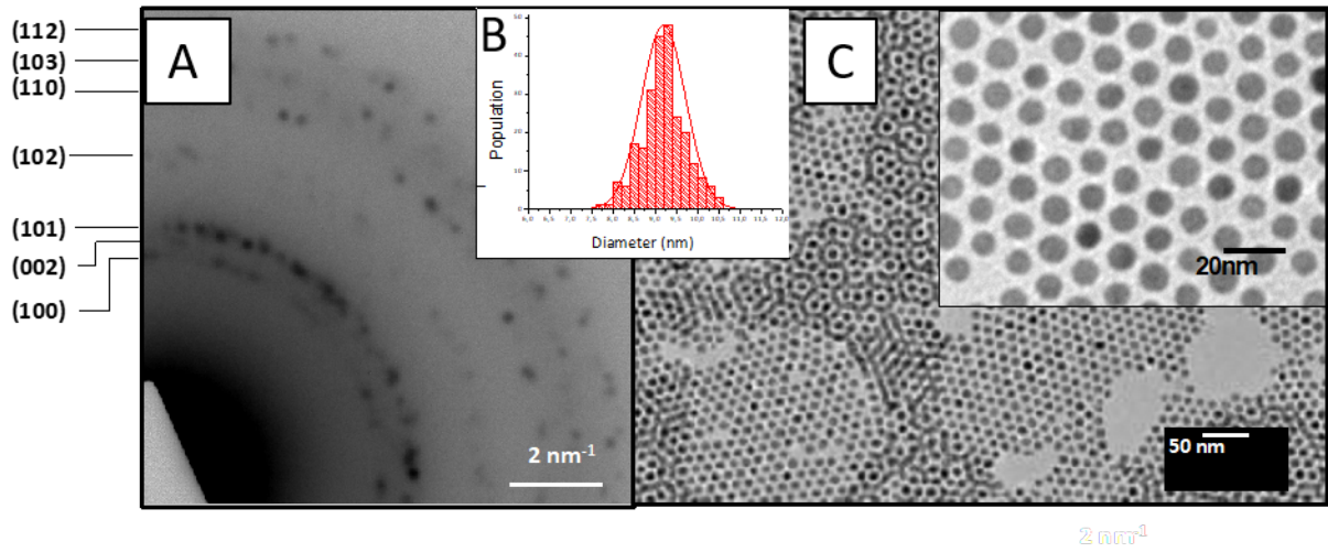
Figure 5: TEM characterization of 9.2 nm hcp cobalt nanoparticles. (A) SAED, (B) size histogram, (C) TEM images.
