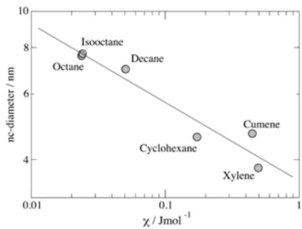
Figure 3 : Log-log plot of the experimental cobalt nanoparticle size and the interaction parameter.
