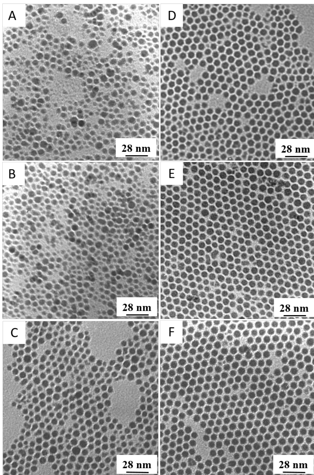
Figure 1 : TEM images of cobalt nanoparticles synthesized at various sodium tetrahydroboride concentrations, R. A (R=0.5), B (R=1), C (R=2), D (R=4), E (R=6) and F (R=8). In insert, TEM images obtained at a lower magnification.
