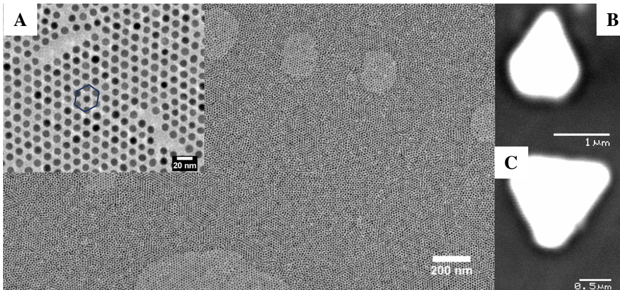
Figure 10. 9.2 nm spherical cobalt nanoparticles with 6% polydispersity self-organized in (A) 2D and thin 3D assemblies as obtained by drop deposition on amorphous carbon. B and C) superlattices obtained by slow evaporation at room temperature on graphite substrate.
