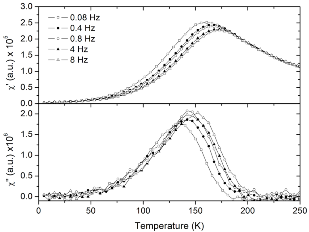
Figure 14 : (A) In phase and (B) out of phase part of the ac susceptibility versus temperature, measured at frequencies between 0.08 and 8 Hz of a supercrystalline film of 8 nm-Co nanoparticles.
