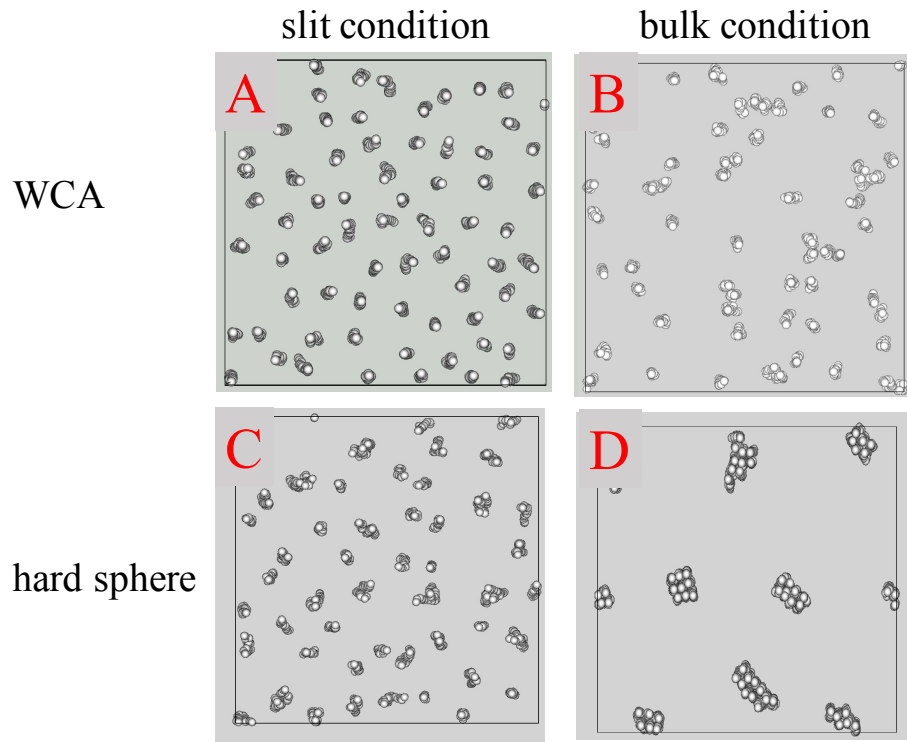
Figure 19. Snapshots of configurations for a confined dipolar fluid at \mu=3.0 , \rho=0.1 , T=1.0 , L=20 and H=40 . In the first and second line the repulsion corresponds to the Week-Chandler-Anderson (WCA) or the hard sphere potential. On the left side, slit conditions apply for the simulation box, while on the right side periodic bulk conditions are used.
