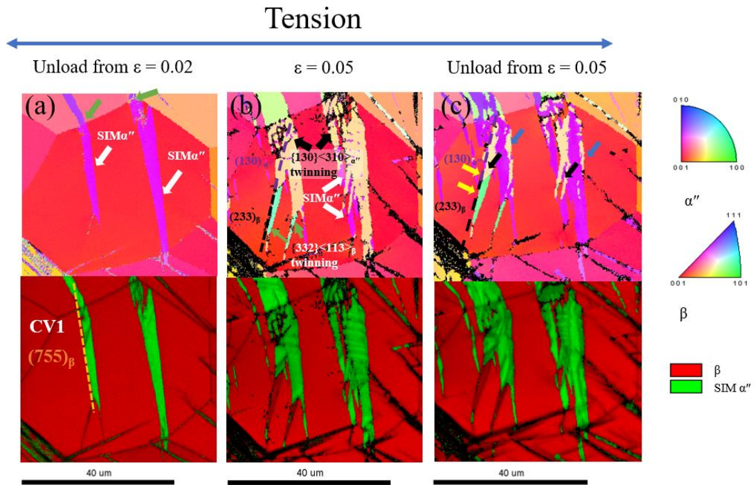
Figure 3. inverse pole figure maps and phase + IQ maps of grain with orientation II taken from the same region at strain steps of (a) \epsilon=0.02 , (b) 0.05 (holding tensile stress), and (c) 0.05 (stress released).
