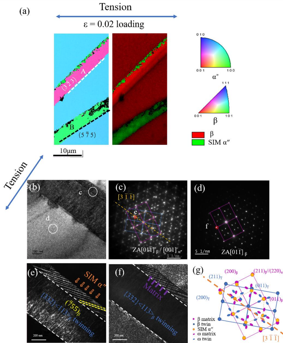
Figure 2. EBSD and TEM investigations at grains with orientation I: (a) invers pole figure maps and phase + IQ maps of the deformed sample taken at \epsilon=0.02 (holding tensile stress); (b) bright-field image of a \{332\}\langle 113\rangle with interfacial SIM \alpha'' in sample taken at \epsilon=0.05 (unloading), (c-d) diffraction pattern taken from region indicated by circle in (b), (e) and (f) corresponding dark-field images of one variant of SIM \alpha'' and of the \beta matrix, respectively, and (g) key diagrams corresponding to the diffraction pattern in (c).
