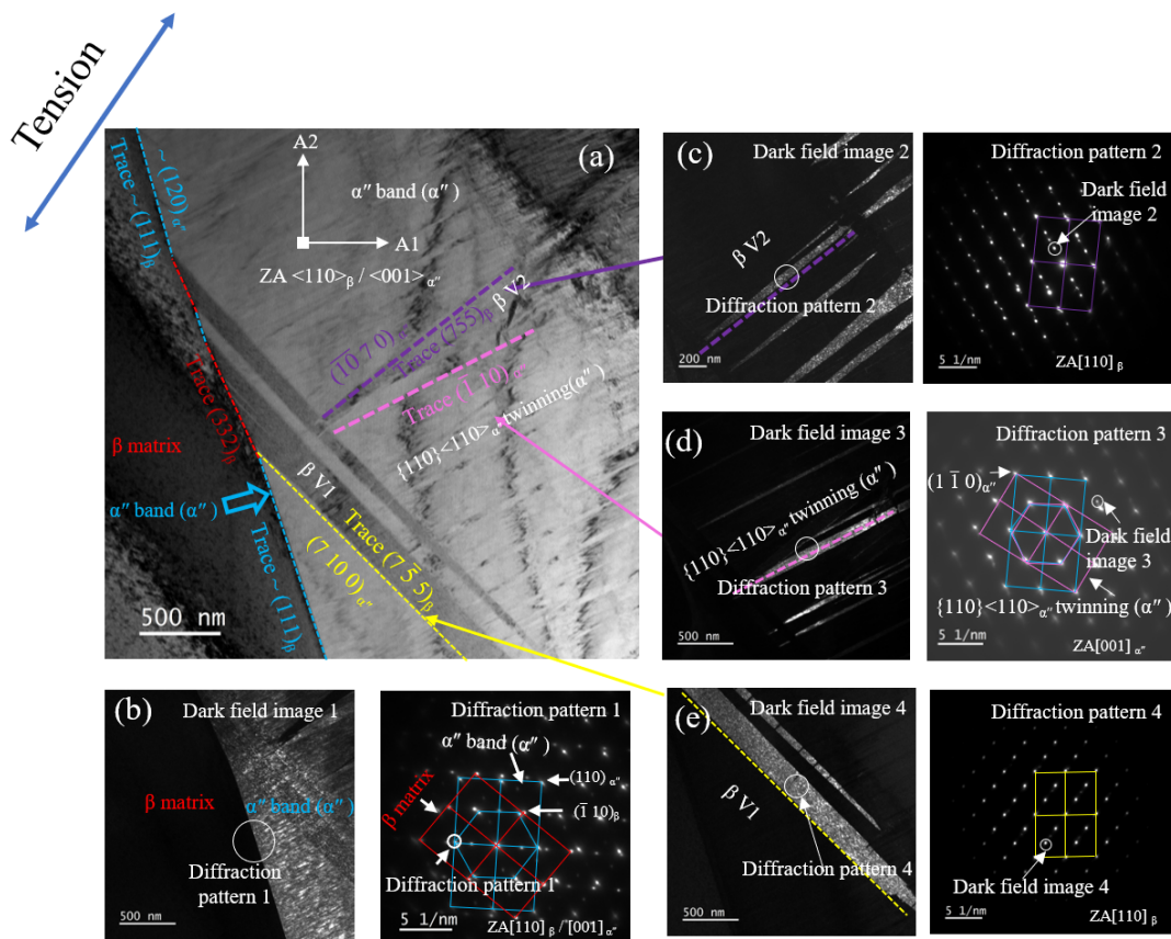
Figure 4 TEM observations of a grain with orientation II in a specimen strained to 0.05 and unloaded. Micrographs of (a) bright field image, (b-e) dark field images and their corresponding diffraction patterns (DP) associated by arrows to the locations of the interfaces.
