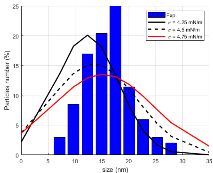
Figure 7: Experimental and simulated size distributions.
