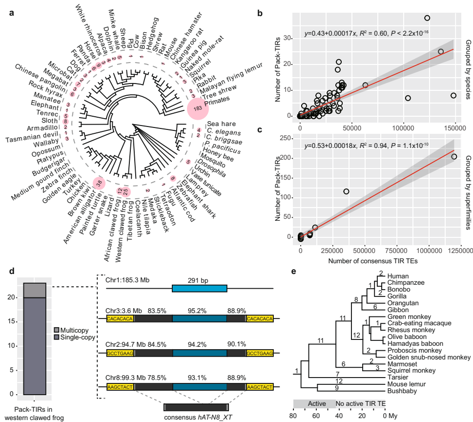
Fig. 1 Pack-TIRs detected in the animal reference genomes. a Distribution of Pack-TIRs in 100 animals. The number of Pack-TIRs (if any) is shown close to the taxon name, and the size of the pink background is proportional to the number. Note: the primate order (18 species) and the Drosophila genus (11 species) are collapsed, and the total number of Pack-TIRs (if present) is shown. b, c Linear relationship between the number of Pack-TIRs and the number of consensus TIR TEs in each species ( b ) or in each TE superfamily ( c ). The shaded areas represent 95% confidence interval. The F -test was used to calculate the P -value. d Pack-TIRs in western clawed frog. The left subpanel shows the number of multicopy and single-copy Pack-TIRs, and the right subpanel shows one case harboring three transposition events with the parental copy (light blue) shown at the top, TIR TE shown at the bottom and the correspondence between TE and Pack-TIR shown as dashed lines. The percentages represent sequence identities relative to the parental copy and the consensus TE. TIRs, non-TIR TE sequences, and internal non-TE sequences are shown in gray, black, and dark blue, respectively. The target site duplications (TSDs) in flanking regions are also marked in yellow. Abbreviations such as “Chr1: 185.3 Mb” indicate a chromosomal coordinate, with Mb representing the number of mega bases. e Emergence of Pack-TIRs along the phylogenetic tree of primates. Two periods with active or inactive TIR TEs are marked along the evolutionary time. “My” represents million years.
