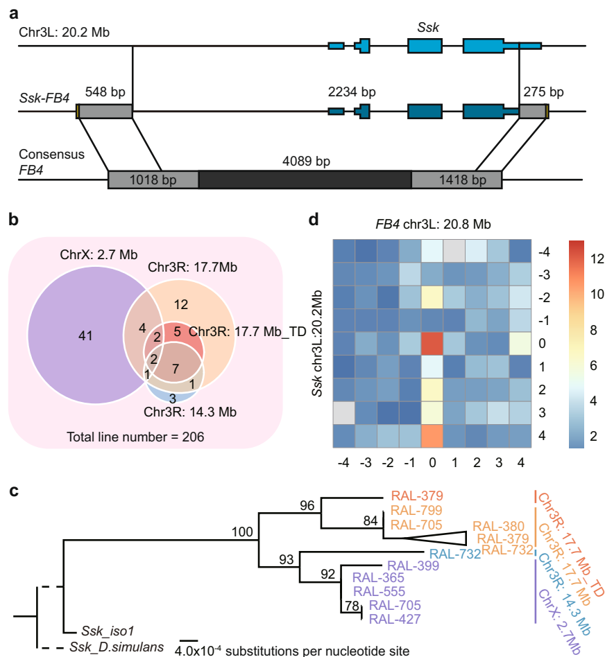
Fig. 3 Origin and spread of Ssk-FB4s in Drosophila populations. a Schematic show of the Ssk-FB4 gene structure. The figure convention follows that of Fig. 1d with the exception that the thinner boxes, the thicker boxes, and the intervening lines represent the UTR, coding exons, and introns of Ssk , respectively. b Venn diagram showing the numbers of lines harboring different Ssk-FB4 copies. “TD” represents the tandemly duplicated copy at chr3R: 17.7 Mb. Note: some lines contain more than one copy. c Phylogenetic tree of Ssk-FB4s and Ssk . The genomic sequences of Ssk in the reference strain of D. melanogaster and the closely related species D. simulans were used as the outgroups. Ssk-FB4s sequenced in a set of Drosophila lines served as ingroups with the colored IDs referring to individual DGRP lines (e.g., RAL-379). Branches with bootstrap scores lower than 60 were collapsed. The ancestral branch of Ssk-FB4s and Ssk and the branch leading to D. simulans are shown as dashed lines because the exact length could not be polarized without outgroups. Four copies of Ssk-FB4 were color-coded. d Chromosome conformation capture (Hi-C) data of Ssk (Y-axis) and FB4 at chr3L: 20.8 Mb (X-axis). The flanking regions of both loci are shown such that each bin represents a 10-kb window and bin 0 indicates Ssk and FB4 . In total, a 90-kb region was covered. The normalized interaction strength is color-coded.
