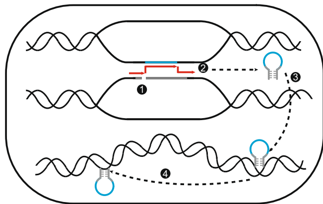
Fig. 6 Working model of FoSTeST. The model includes four steps: (1) replication fork stalling; (2) template switching; (3) transposition; and (4) potential amplification via a new round of transposition.
