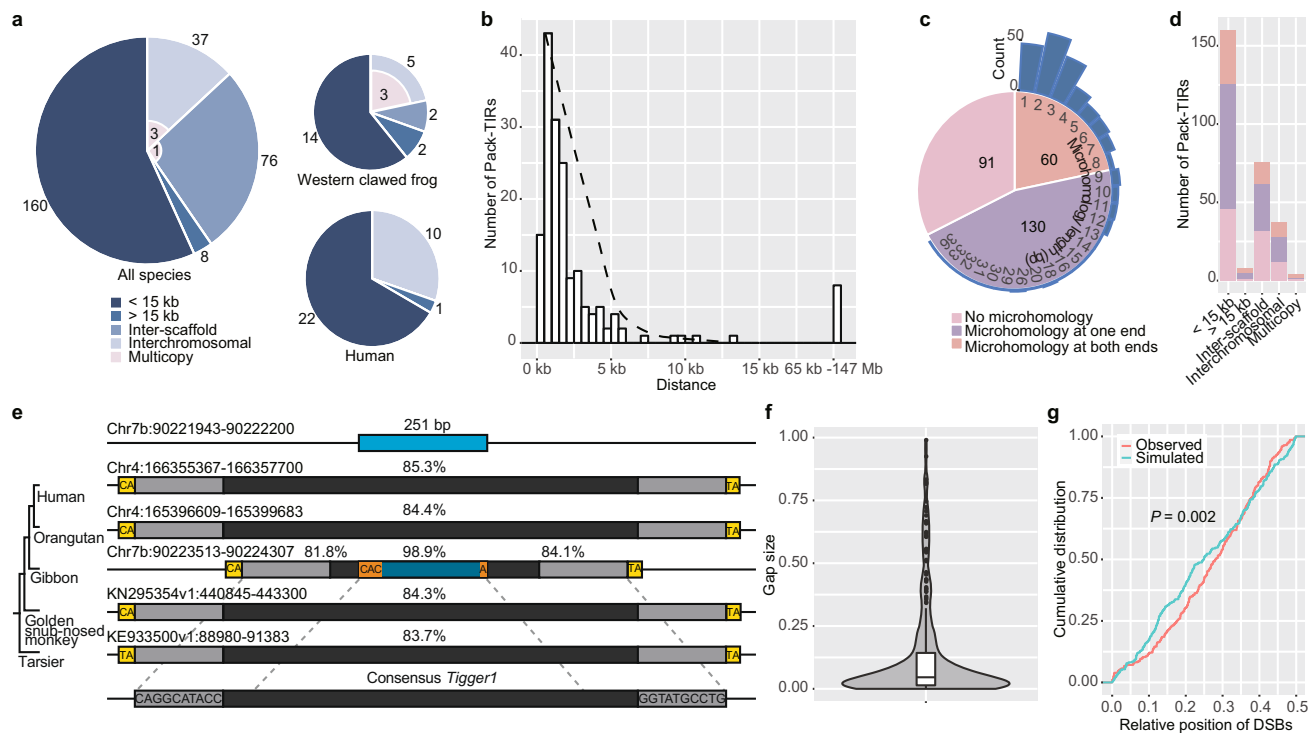
Fig. 2 Evidence supporting the gap-filling model for the generation of single-copy Pack-TIRs. a Distribution of Pack-TIRs classified by distance from their parental copies. The pie charts show the statistics for all species, western clawed frogs, and humans, respectively. Numbers of multicopy Pack-TIRs are highlighted in pink. For example, three out of five interchromosomal Pack-TIRs are multicopy in western clawed frogs. b Histogram of intrachromosomal Pack-TIRs in terms of distance to their parental copies. The dashed curve shows the lowest fitting result. c Distribution of Pack-TIRs classified by the presence of microhomology at breakpoints. The sidebar shows the histogram of the microhomology length. d Distribution of Pack-TIRs with respect to the microhomology presence at breakpoints. Single-copy Pack-TIRs close or far from parental copies and multicopy Pack-TIRs are separately counted. e A comparative view of a demo Pack-TIR in gibbons (case #144 in Supplementary Data 1). To simplify, in addition to gibbons, only four phylogenetically representative primates are shown. The figure convention follows Fig. 1d except that the microhomology is marked in orange. Note that the left TSD was mutated from TA to CA in the ancestor of humans and monkeys. f Proportion of each gap ( n = 281 samples) relative to the corresponding consensus TE. The distribution is shown as a violin plot: the box indicates the median (middle line) and the interquartile range (IQR, box limits); outliers are beyond 1.5 times IQR; and the violin curve indicates the probability density of the data. g Cumulative density distribution of the observed and simulated relative positions of breakpoints to consensus TEs. Values closer to 0.5 at X-axis indicate positions closer to the middle of the TEs, whereas values close to 0 indicate positions closer to the terminals. The two-sided Kolmogorov-Smirnov test was used to calculate the P -value.
