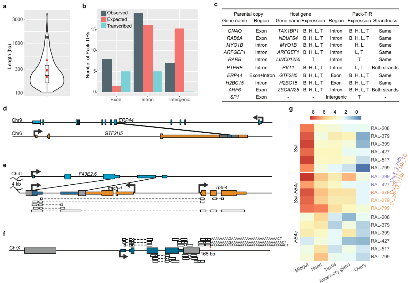
Fig. 4 Sequence and transcriptional features of Pack-TIRs. a Length distribution of the internal sequences ( n = 281 samples). The distribution is shown as a violin plot in Fig. 2f. The four red dots represent the multicopy Pack-TIRs. b Distribution of parental sequence types in humans. “Observed” shows the actual numbers of Pack-TIRs divided by the functional types of their parental sequences; “Expected” shows the numbers calculated based on the proportion of all annotated exons and introns; and “Transcribed” shows the numbers of transcribed Pack-TIRs in each category. c Transcribed human Pack-TIRs. Host genes indicate the genes into which Pack-TIRs were inserted. “B”, “H”, “L”, and “T” indicate the brain, heart, liver, and testis, respectively. d One human example showing 3’ UTR chimerism. The figure convention follows that of Fig. 1d with the exception that the host gene is marked in orange and the transcription direction is shown by thick arrows. e One worm example showing 5’ UTR chimerism. The parental gene is close to the host gene at a 4-kb distance. The boxes connected by dashed lines indicate the spliced RNA-seq reads. Blank arrows indicate paired-end Illumina short reads. The bottom long read was generated on the Nanopore platform (“Methods”). Note: mtch-1 and rpb-4 are divergently transcribed. f Gene structure of Ssk-FB4 in D. melanogaster at chrX: 2.7 Mb. Ssk-FB4 is highly transcribed in the midgut, and only a few representative spliced reads spanning breakpoints between the internal sequence and TE and reads supporting continuous transcription toward 165-bp (marked by a red dashed line) downstream regions are shown. Note: the reads containing poly(A) tails have non-A residues, consistent with a previous report 46 . g Heatmap showing the expression profile of Ssk , Ssk-FB4s , and FB4s in five tissues in D. melanogaster . The expression levels were quantified as \log_2 transformed TPM (transcripts per million mapped reads, n = 2 biologically independent replicates).
