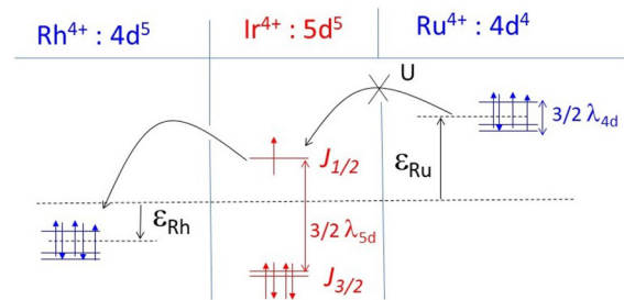
FIG. 1. Sketch of the ionic t_{2g} levels for Rh, Ir, and Ru. SOC splits them into one J_{1/2} and two J_{3/2} levels ( J_{3/2-m_j} with m_j = \pm 1/2, 3/2 ), with a much larger value for Ir, being a 5d TM, than Rh and Ru ( \lambda_{5d} \simeq 0.5 eV vs \lambda_{4d} \simeq 0.1 eV). We assume a shift \epsilon between Ir and the other TM (see Fig. 4 for a discussion of its origin). Electrons should be transferred to the lowest available energy level, unless the Coulomb repulsion U forbids double occupation.
