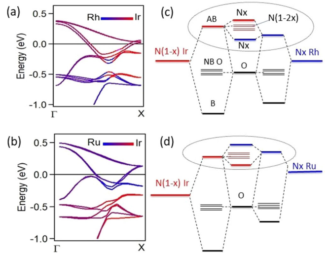
FIG. 4. (a) Band structure calculated for an ordered structure \text{Sr}_2(\text{IrRh})_{0.5}\text{O}_4 along \Gamma X , without SOC. The color is proportional to the atomic character (red-blue scale). (b) Same for Ru. [(c), (d)] Sketch of the energy levels of oxygen, Ir, and TM dopant and their relative hybridization, based on calculation presented in the Supplemental Material, but not to scale. The hybridized states have mixed atomic character, and their color indicates the dominant one. The circled part represents hybridization of N levels, from Ir and TM.
