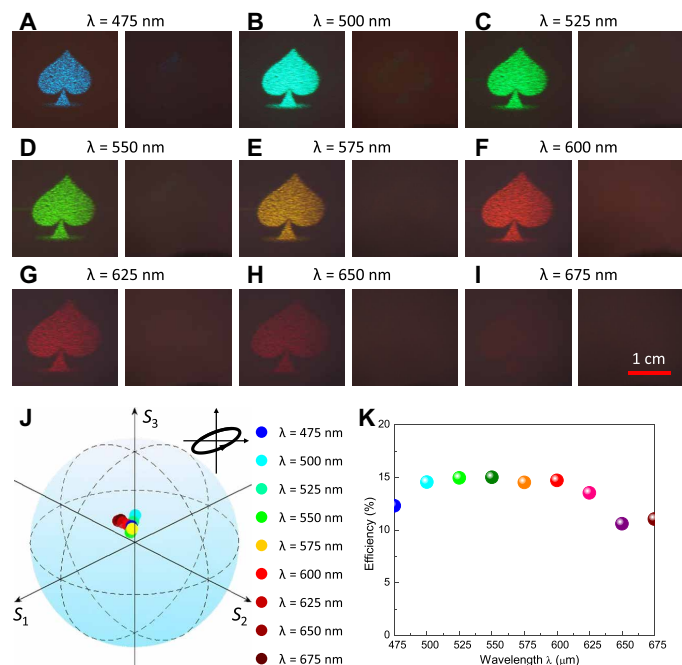
Fig. 5. Broadband polarization-maintaining properties of the nondispersive metasurface. (A to I) Measured holographic images with the incident wavelength from 475 to 675 nm (left: without analyzer; right: with broad band quarter wave plate at \theta_{LP} = 49.07^\circ and linear polarizer (LP) at \theta_{LP} = 49.07^\circ to block the holographic images). The holographic images in the right panels are almost totally blocked in the entire visible range, confirming the exceptional broadband response of out polarization-maintaining design approach. (J) Measured SoP at different wavelengths agrees well to the designed value in Fig. 2G. (K) Measured efficiency is higher than 10% across the entire visible range.
