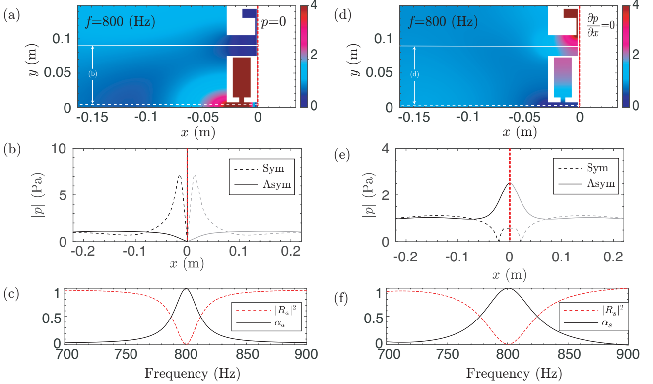
FIG. 4. (Color online) Critical coupling of the symmetric and antisymmetric problem. (a) Represents the absolute value of the total acoustic pressure field at the perfect absorption of the antisymmetric problem. (b) Shows the absolute value of the total pressure field, |p| , along the profiles shown in (a) considering the field in each slit for the antisymmetric problem. (c) Shows the reflection and the absorption coefficient of the antisymmetric problem. (d) Represents the absolute value of the total acoustic pressure field at the perfect absorption of the symmetric problem. (e) Shows the absolute value of the total acoustic field, |p| , along the profiles shown in (c) considering the field in each slit for the symmetric problem. (f) Shows the reflection and the absorption coefficient of the symmetric problem.
