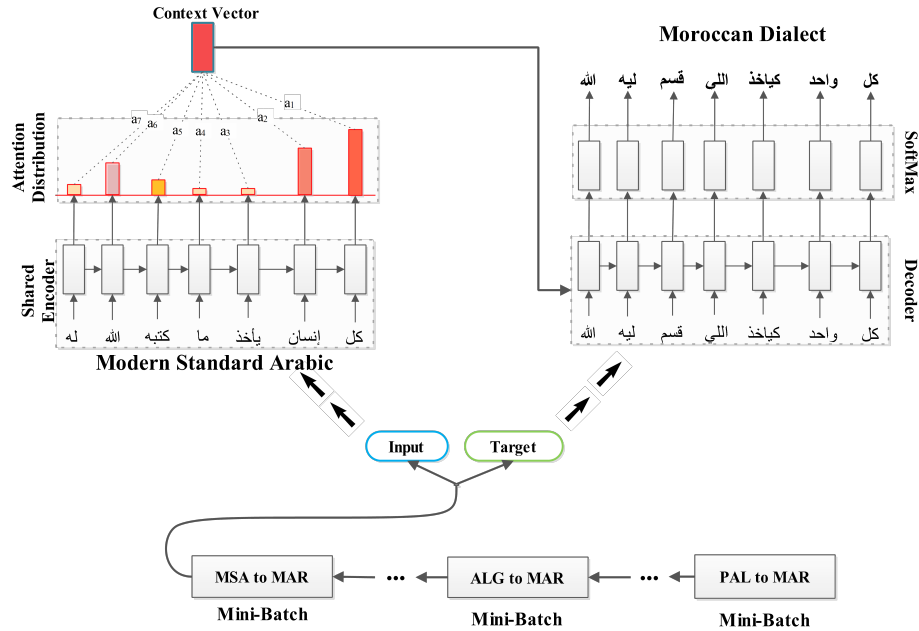
Fig. 1. Illustration of the architecture of the used multitask sequence-to-sequence learning with an attention mechanism. The model takes a mini-batch of data from each language pair.
