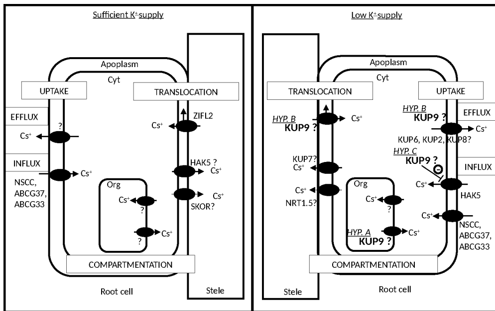
Figure 6: Model for \text{Cs}^+ transport in roots of A. thaliana depending on the level of \text{K}^+ supply. INFLUX. As for other cations, \text{Cs}^+ taken up by plants from the soil solution is transported across the root mainly through the symplastic pathway. Non-selective Cation Channels (NSCC, White and Broadley 2000, Hampton et al. 2005) and the high-affinity \text{K}^+ transporter HAK5 (Qi et al. 2008) are thought to mediate the major part of \text{Cs}^+ influx in sufficient (mM range) and low ( \mu\text{M} range) \text{K}^+ conditions respectively. ABCG37 and ABCG33 mediate a significant part of \text{Cs}^+ influx regardless the \text{K}^+ level (Ashraf et al., 2021). TRANSLOCATION. \text{Cs}^+ is highly mobile within plants. From the roots, \text{Cs}^+ is loaded into the xylem and distributed towards the aerial parts through yet unidentified transport systems. The Major Facilitator Superfamily transporter ZIFL2 has been proposed to prevent \text{Cs}^+ xylem loading mediating \text{Cs}^+ release into the apoplast of endodermis and pericycle, under \text{Cs}^+ and \text{K}^+ excess (Remy et al. 2015). COMPARTMENTATION. Regarding its intracellular distribution, analyses of contaminated plant cells revealed that \text{Cs}^+ is not limited to the cytosol but is also found in vacuole and probably chloroplasts (Le Lay et al. 2006, Akamatsu et al. 2014). Identities of transport systems involved in these mechanisms are unknown. EFFLUX. Given our results, we propose three hypotheses involving KUP9 in the limitation of \text{Cs}^+ accumulation (see in text) either speculating that KUP9 could work as an efflux carrier (HYP. A and B) or that KUP9 could affect transport of \text{Cs}^+ through others carriers (HYP. C).
