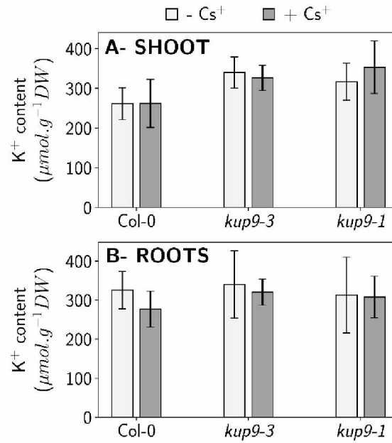
Figure S3: K + content in Cs + -exposed plants. K + content was measured in 30 days-old plants supplied during 12 days with a nutrient solution containing 10 \mu\text{M} K + and exposed during 7 days to 1 \mu\text{M} Cs + (+ Cs + ) or not exposed (- Cs + ). Data for (A) Shoot and (B) Roots are means \pm SD (n=11-12). ANOVA analyses performed to compare K + content between lines for each level of K + supply revealed no significant differences.
