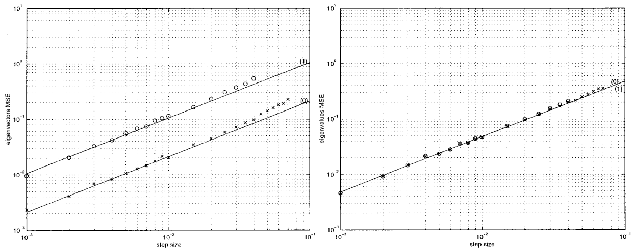
Fig. 2. Estimated [respectively, theoretical asymptotic] eigenvalues and eigenvectors MSE as a function of the step size \gamma when the CS structure is taken into account ( \times ) [respectively, (0)] or not (o) [respectively, (1)].
