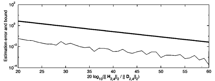
Fig. 1. Estimation error bound (10) (thick line) and measured error.
