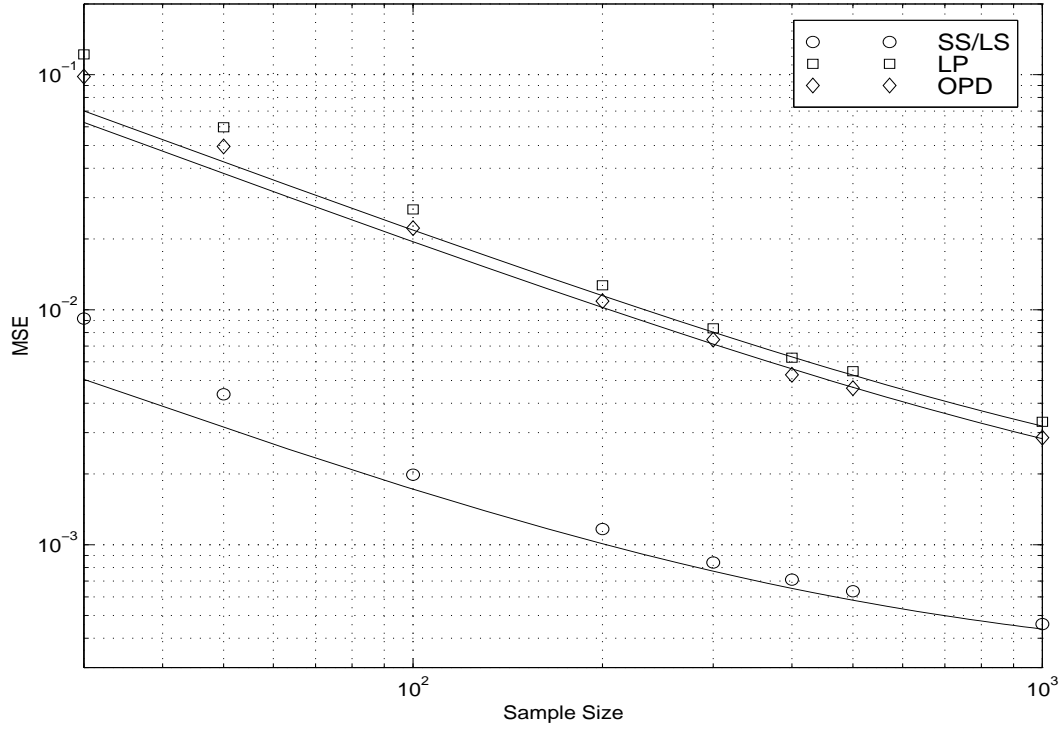
Fig.3 MSE of \hat{\mathbf{h}}_2 versus the sample size for \mathbf{h}_2 given by (5.1), a signal noise ratio of 17dB and for \|\mathbf{d}_{2,12}\| = 0.05 .
