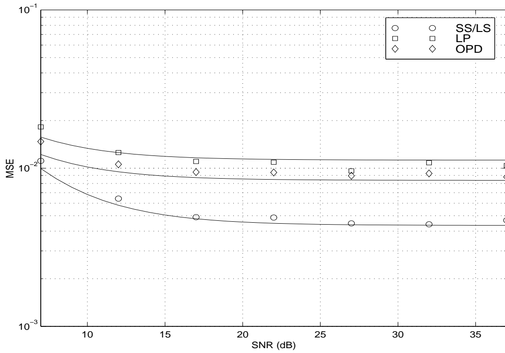
Fig.6 MSE of \hat{\mathbf{h}}_2 , for N = 300 and \|\mathbf{d}_{2,12}\|^2 = 0,01 , versus the signal to noise ratio.
