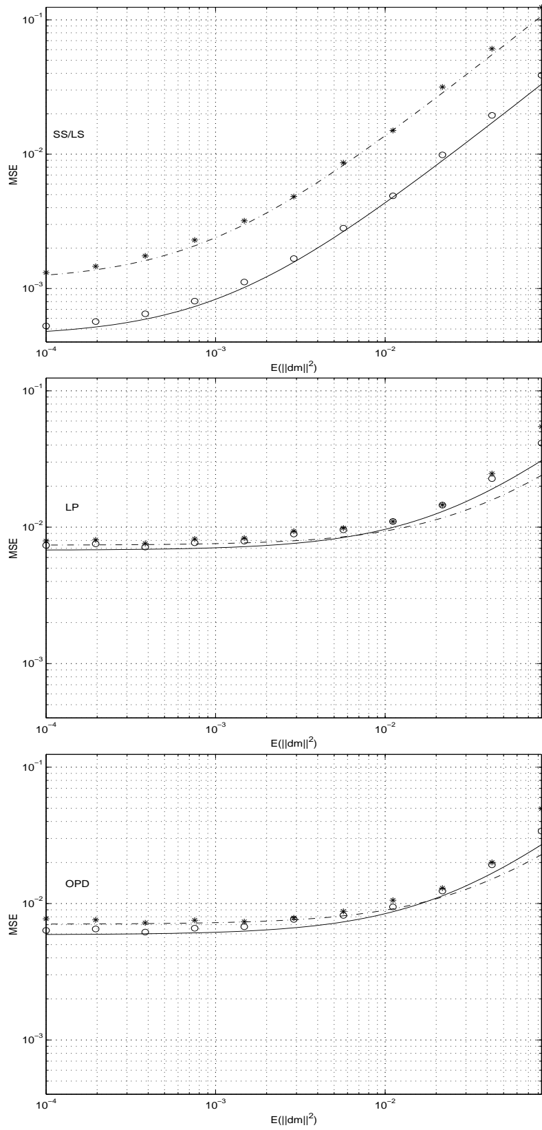
Fig.7 MSE of \hat{\mathbf{h}}_2 , for N = 300 and \text{SNR}=17\text{dB} , versus \sigma_d^2 for respectively \mathbf{h}_2 given by (5.1) (o)(—) and (5.2) (*- - -).
