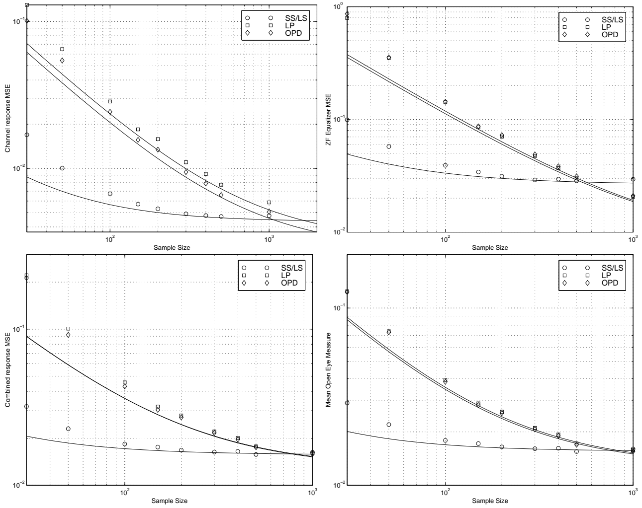
Fig.8 MSE of \hat{\mathbf{h}}_2 , \hat{\mathbf{g}}_{2,2}^{\text{ZF}} , \hat{\mathbf{f}}_{2,2} and \text{OEM}(\hat{\mathbf{f}}_{2,2}) for SNR=17dB, versus the sample size for \sigma_d^2 = 0.0111 and \mathbf{h}_2 given by (5.1).
