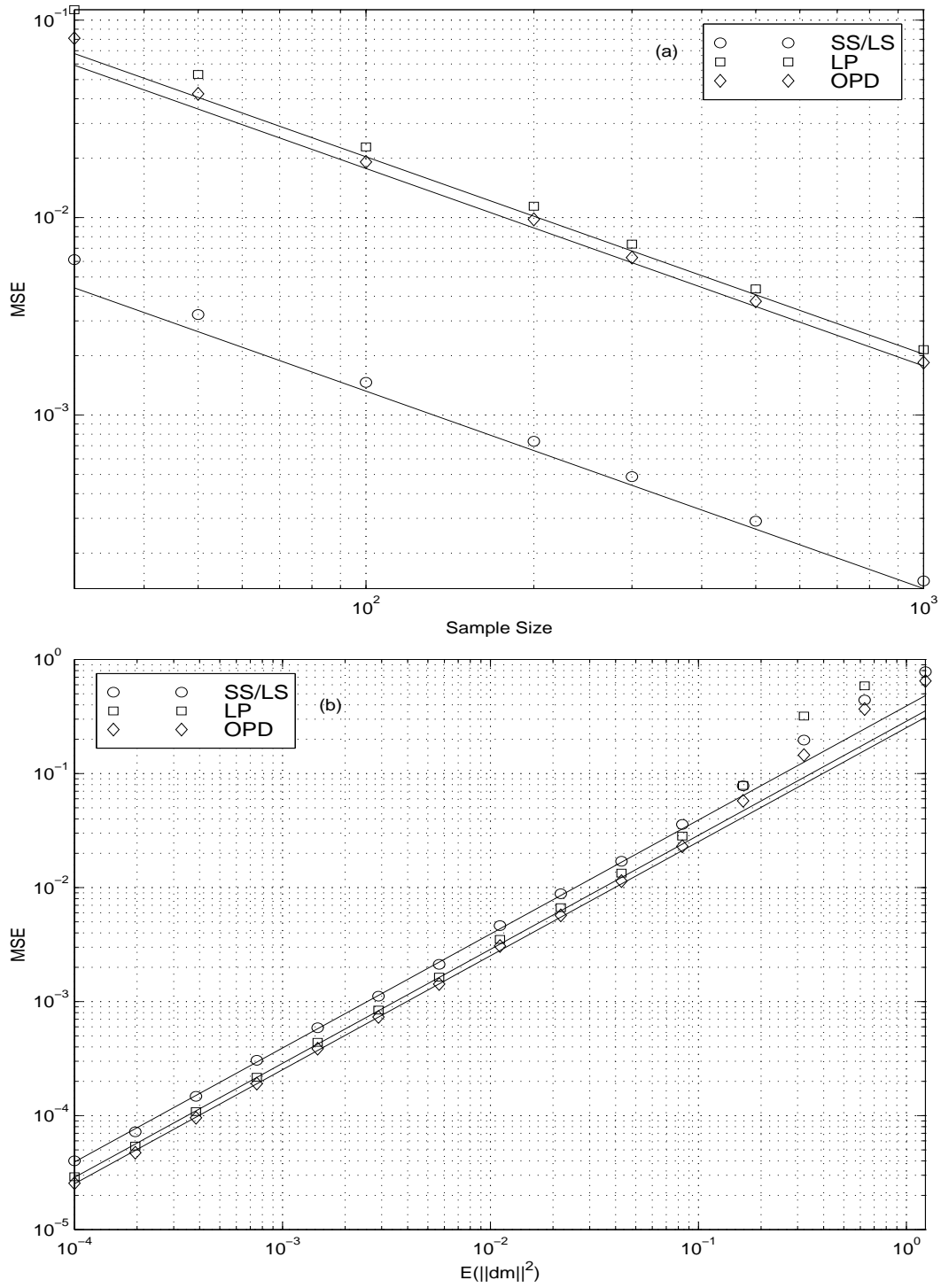
Fig.5 MSE of \hat{\mathbf{h}}_2 , for no tails, versus the sample size (a), and for exact statistics versus \sigma_d^2 = E(\|\mathbf{d}_{2,12}\|^2) (b).
