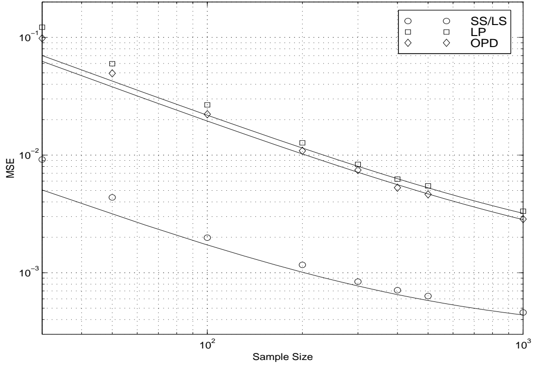
Fig.3 MSE of \hat{\mathbf{h}}_2 versus the sample size for \mathbf{h}_2 given by (5.1), a signal noise ratio of 17dB and for \|\mathbf{d}_{2,12}\| = 0.05 .
