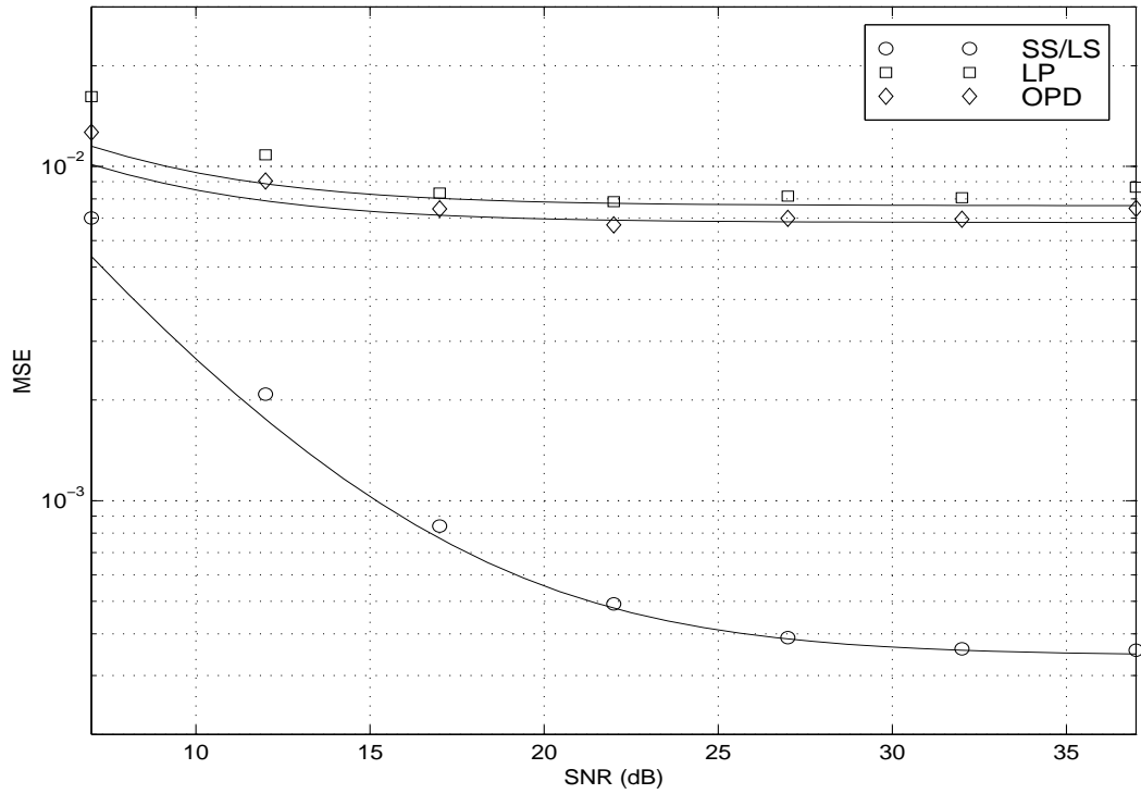
Fig.4 MSE of \hat{\mathbf{h}}_2 versus the signal to noise ratio, for N = 300 and \mathbf{h}_2 given by (5.1) and for \|\mathbf{d}_{2,12}\| = 0.05 .
