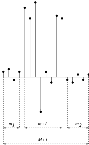
Fig. 2. Channel response with small heading and trailing terms
