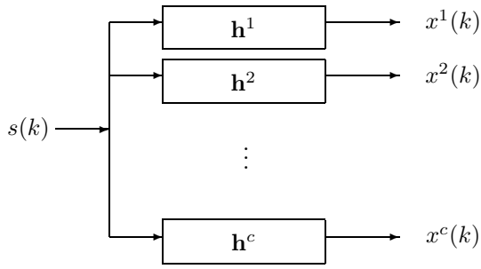
Fig. 1. Single input multiple output channel
