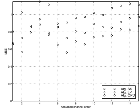
(b) Blind identification error
