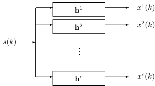
Fig. 1. Single input multiple output channel
