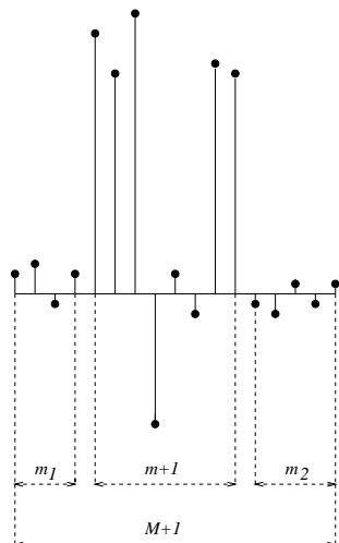
Fig. 2. Channel response with small heading and trailing terms
