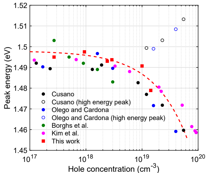
FIG. 2. Peak position energy as a function of the hole concentration. Our CL spectra are compared to available literature data from Cusano for 20 K CL of GaAs single crystal slices [30], Olego and Cardona for 4 K PL of Zn-doped single crystal GaAs [6], Borghs et al. for 30 K PL of MBE-grown Be-doped GaAs [31] and Kim et al. for 12 K PL of MOCVD-grown C-doped GaAs [32]. The red dashed line is a guide to the eyes.
