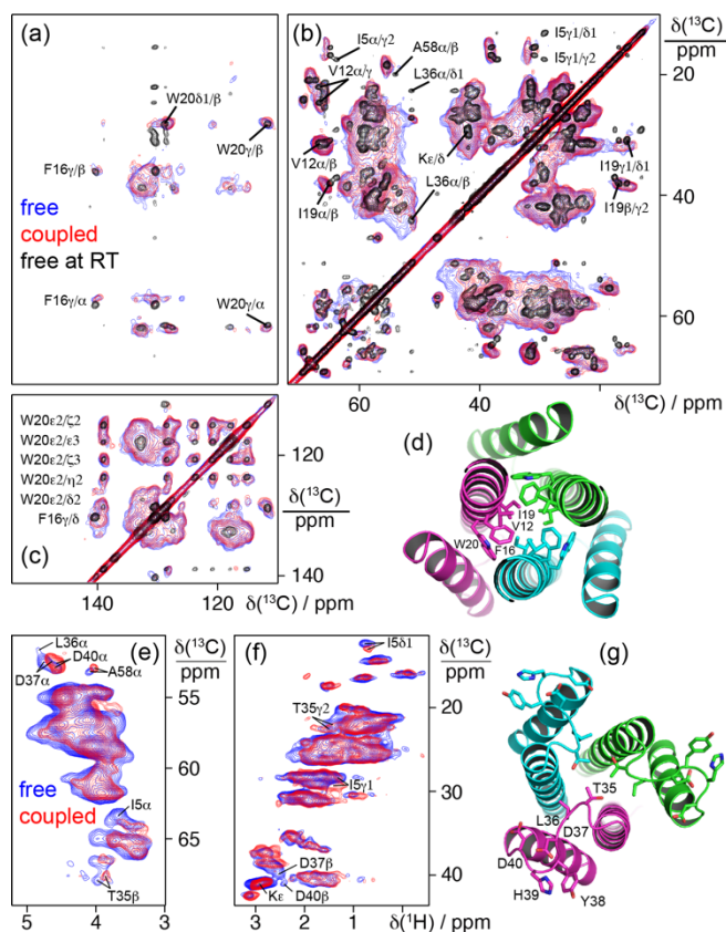
Figure 4. Comparison of free and VLP-coupled LAH antigen. (a), (b) and (c) Overlays of different spectral regions from DNP-enhanced 2D CORD spectra of ^{13}\text{C} , ^{15}\text{N} -labeled free (blue) and VLP-coupled (red) LAH antigen at 800 MHz and 115 K with 40 kHz MAS with the room temperature 2D DARR spectrum of free LAH antigen (black) at 800 MHz with 20 kHz MAS. (d) Crystal structure of LAH antigen showing the side chains of V12, F16, I19 and W20 that make up the hydrophobic core of the trimer. (e) and (f) Overlays of ^1\text{H} - ^{13}\text{C} and ^1\text{H} - ^{15}\text{N} -labeled free (blue) and VLP-coupled (red) LAH antigen at 1 GHz with 60 kHz MAS. (g) Crystal structure of LAH trimer showing the side chains of residues T35-D40 in the loop between helices 1 and 2.
