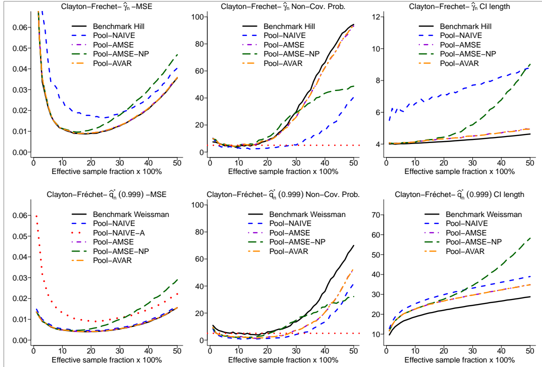
Figure D.4: As in Figure D.2, in the Clayton-Fréchet model (c).
