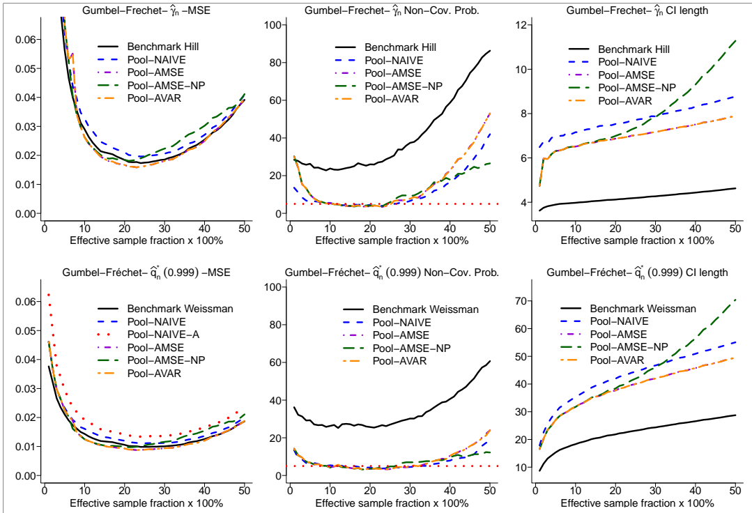
Figure D.5: As in Figure D.2, in the Gumbel-Fréchet model (d).
