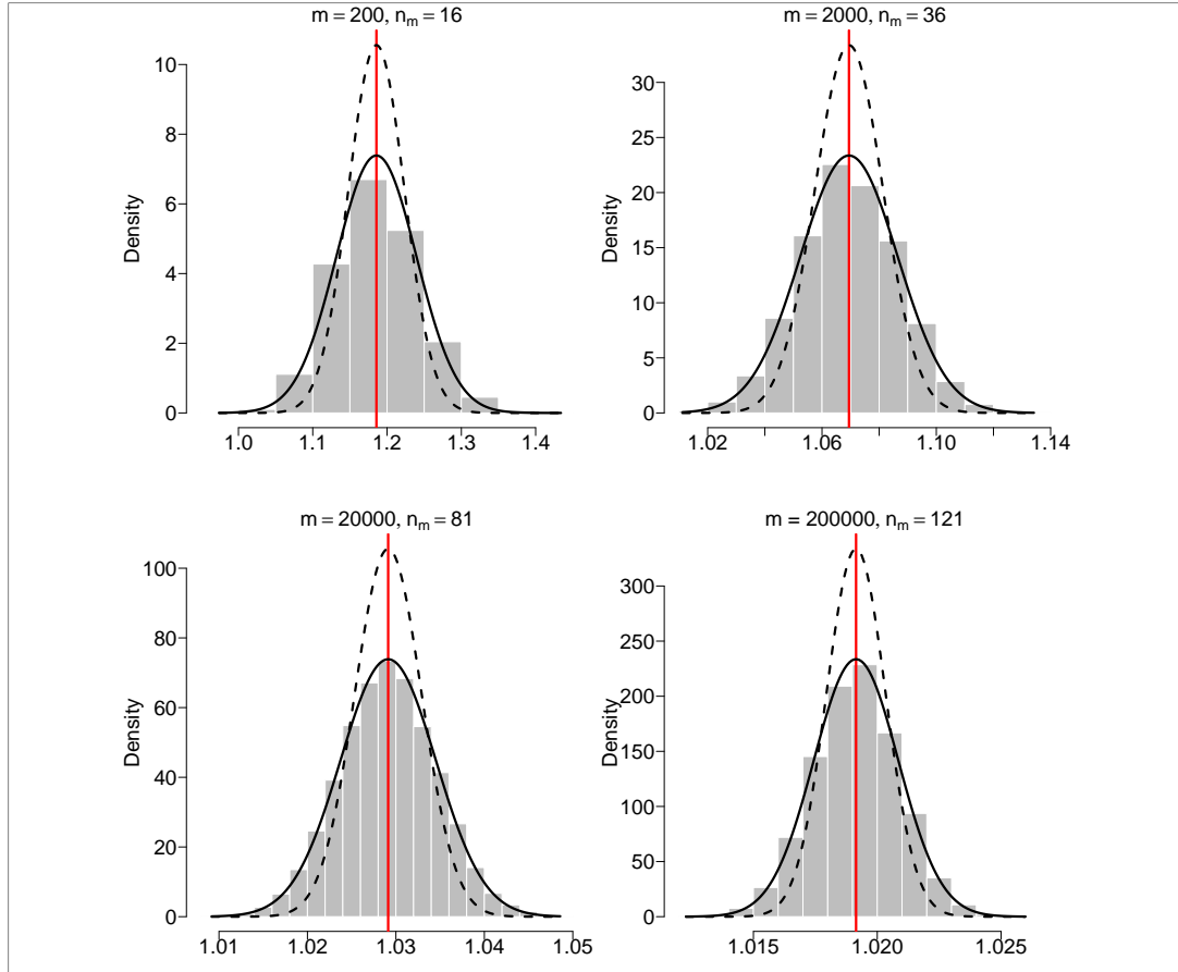
Figure C.1: Empirical distribution of the naive distributed Hill estimator in the simulation setup described in Section C.5. Top left: m = 200 , top right: m = 2,000 , bottom left: m = 20,000 , bottom right: m = 200,000 . The red vertical line represents the mean of the distributed Hill estimates, and the dashed (resp. solid) line represents the normal density curve with mean \bar{y} (i.e. the empirical mean of the distributed Hill estimates) and variance 1/k (resp. 49/(24k) ).
