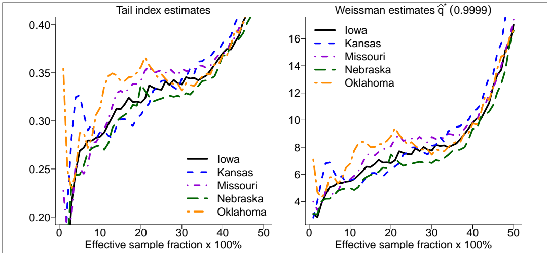
Figure D.22: Car insurance data: Hill estimates \hat{\gamma}_j(k_j) (left) and Weissman estimates \hat{q}_j^*(0.9999|k_j) (right) for each state, as functions of the sample fraction k_j/n_j , assumed to be identical in each sub-sample.
