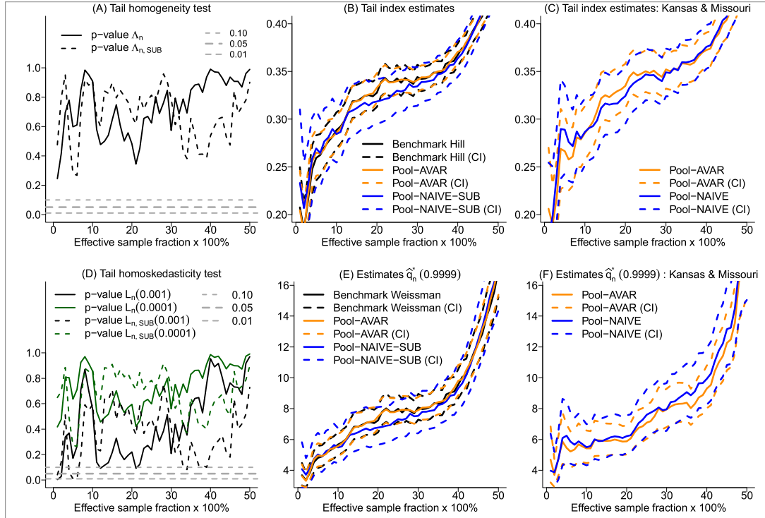
Figure 1: Car insurance data. In (A) and (D), \Lambda_{n, \text{SUB}} and L_{n, \text{SUB}}(p) denote the test statistics \Lambda_n and L_n(p) calculated from the subsampled data of total size 5 \times 700 = 3,500 . In (B) and (C), Pool-AVAR and Pool-NAIVE respectively denote the variance-optimal pooled estimator and the naive pooled estimator of the tail index. In (E) and (F), Pool-AVAR and Pool-NAIVE respectively denote the variance-optimal pooled quantile estimator \hat{q}_n^*(1-p|\hat{\omega}_n^{(\text{Var})}) and its unweighted analog. Pool-NAIVE-SUB stands for these estimators calculated on the subsampled data. All estimates are represented as functions of the sample fraction k_j/n_j , assumed to be identical for each j .
