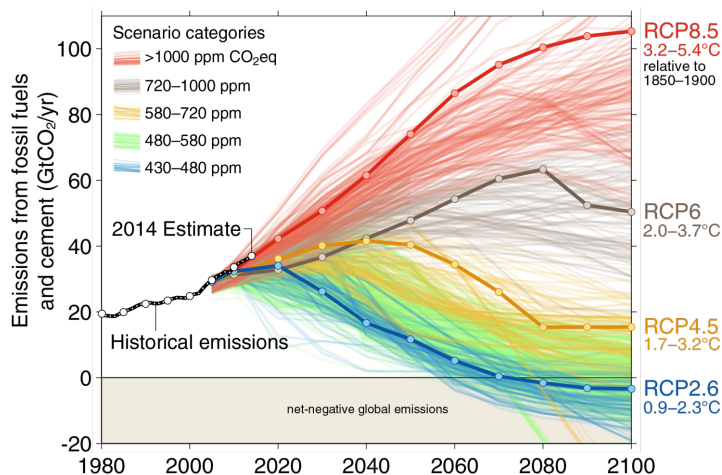
Figure 2. Emissions from fossil fuels and cement (Gt CO 2 /yr) in the Representative Concentration Pathways (RCPs) (lines). Over 1000 IPCC scenario categories from the IPCC 5th Assessment Report are shown, which summarize the wide range of emission scenarios published in the scientific literature and are defined on the basis of CO 2 -eq concentration levels (in ppm) in 2100. The estimate at 2014 is displayed by a red dot, showing that we are currently on the red RCP8.5 pathway. Source: Fuss et al. (2014) [22].
