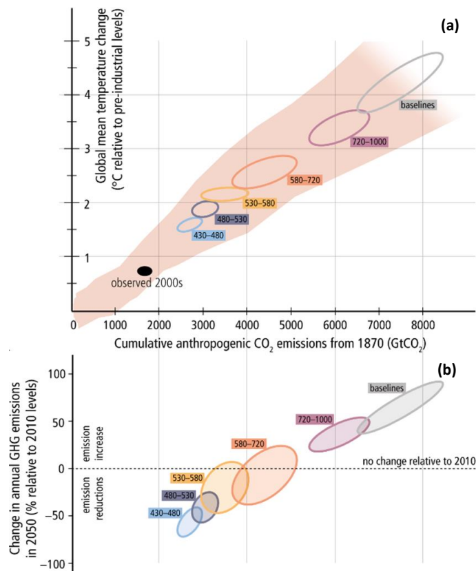
Figure 4. (a) Increase in the average global surface temperature at the time when global CO 2 emissions reach a given net cumulative, plotted against this cumulative, obtained from several data sources. The colored area represents the dispersion of past and future projections obtained using different climate and carbon cycle models taking into account the historical series of emissions and the four RCPs for the entire period up to 2100; it fades as the number of available models decreases. The ellipses represent the ratio between the total anthropogenic warming in 2100 and the cumulative CO 2 emissions from 1870 to 2100, obtained using a simple climate model (median climate response) according to the categories of scenarios used by the WG3. Regarding temperature, the minor axis of the ellipses corresponds to the impact of different scenarios for climatic factors other than CO 2 . The solid black ellipse represents the emissions observed up to 2005 and the temperatures observed during the decade 2000-2009 with the corresponding uncertainties. (b) Relationship between the cumulative CO 2 emissions of the scenario categories and their associated variation in annual GHG emissions by 2050 compared to 2010. Source : IPCC (2013) [8].
