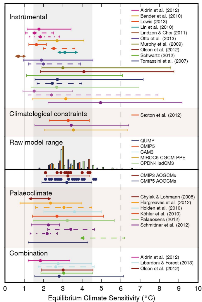
Figure 3. Probability density functions, distributions and ranges for equilibrium climate sensitivity. The grey shaded range marks the likely 1.5°C to 4.5°C range, and the grey solid line the extremely unlikely less than 1°C, the grey dashed line the very unlikely greater than 6°C. Source : IPCC (2013) [8].
