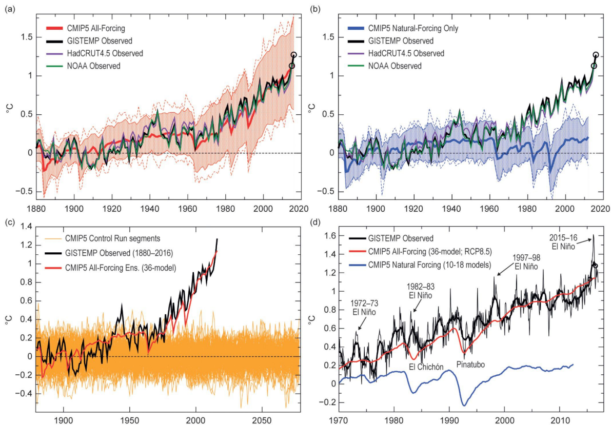
Figure 1. Observed global-mean temperature anomalies vs. Coupled Model Intercomparison Project Phase 5 (CMIP5) simulations ( ^{\circ}\text{C} ; 1881-1920 reference period). (a) CMIP5 All-Forcing (anthropogenic plus natural forcing) grand ensemble mean of individual ensemble means from 36 models (thick red curve); \pm 2 std. dev. (red shading) and minimum-maximum spread (dashed red) of annual means across individual simulations; and observed GISTEMP (black), HadCRUT4.5 (purple) and NOAA (green) anomalies. (b) As in (a) but for natural forcings (18 models; blue curves and shading). (c) Observed (GISTEMP; black) and All-Forcing grand ensemble mean (red) anomalies compared to 200-year segments from 36 CMIP5 control runs (orange). (d) 12-month running mean anomalies for GISTEMP observations (thick black; monthly anomalies are thin black) and CMIP5 All-Forcing (red) and Natural Forcing (blue) grand ensemble means. GISTEMP observed annual means (Jan-Dec) for 2015 and 2016 are highlighted by circles in panels (a), (b), and (d). See also online supplement materials. Source: Knutson et al. (2018) [1].
