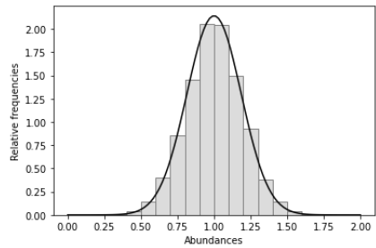
(b) Histogram of the equilibrium abundances.
