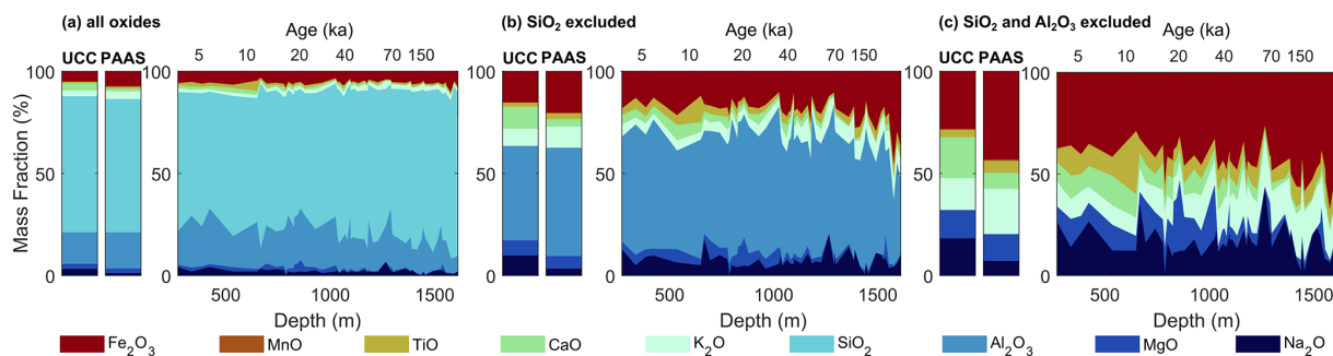
Figure 3. Major element in dust from TALDICE. Data are shown considering all major element oxides (a), excluding SiO 2 (b), and excluding SiO 2 and Al 2 O 3 (c). UCC and PAAS references are shown for comparison (Rudnick and Gao, 2003; Taylor and McLennan, 1985).
