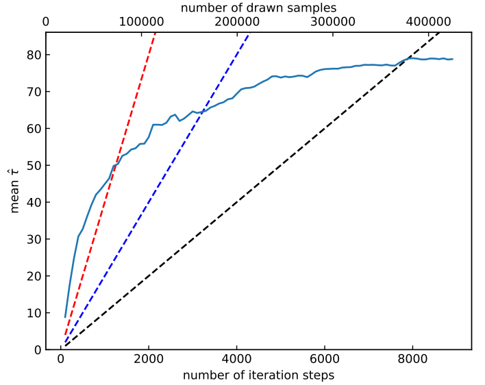
Fig. C.1. Auto-correlation time as function of MCMC iteration steps. The estimated average auto-correlation time \hat{\tau} is shown in blue (solid line). Also shown are the \hat{\tau} = N_{\text{iter}}/20 (red), N_{\text{iter}}/50 (blue), and N_{\text{iter}}/100 (black) lines to indicate different possible levels of acceptance for the model parameter estimates. For this work, the model is considered converged if \hat{\tau} < N_{\text{iter}}/100 and the change in consecutive estimated auto-correlation times \tau is less than 1%.
