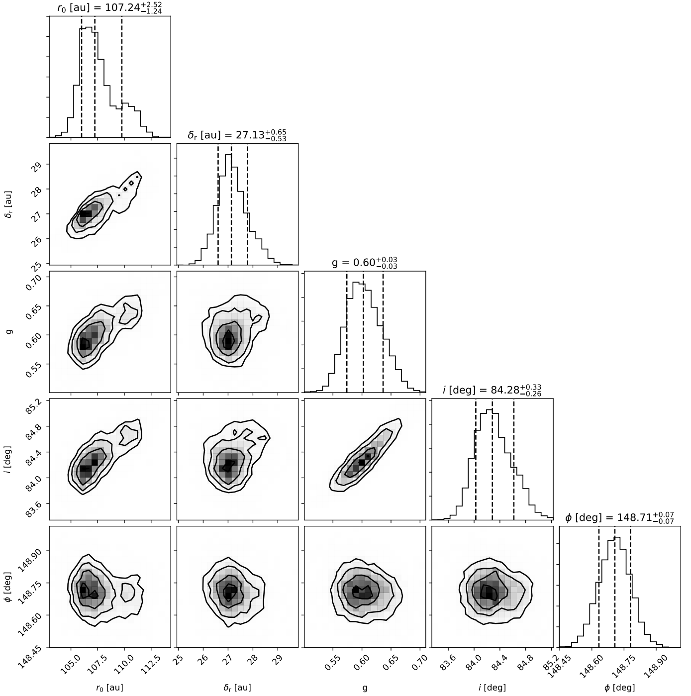
Fig. 4. Projected posterior distribution and density plots of the free parameters used in the disk modeling. The plot additionally shows the 50 %, 16 %, and 84 % quantiles (vertical dashed lines), representing the distributions median and the 1\sigma uncertainties (lower and upper bound), respectively. The 1D histograms represent the probability distributions of each parameter marginalized over the other free parameter. The contour maps represent the central 68.3%, 95.5%, and 99.73% of the 2D probability distributions of different combinations of parameters, marginalized over each other.
