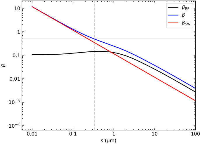
Fig. 11. \beta as a function of grain size. \beta_{RP} and \beta are shown as black and solid lines, respectively. The horizontal solid gray line ( \beta = 0.5 ) is the upper limit for bound trajectories assuming zero eccentricity for the parent body, see Seizestre et al. (2017) for further details. The vertical dashed line indicates the corresponding minimum grain size ( s = 0.34\text{ }\mu\text{m} ) of dust particles required not to be expelled from the disk, assuming a porosity of 70%.
