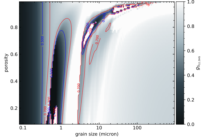
Fig. 7. 2D map of the anisotropic scattering factor g_{S12,DHS} computed at each point of the grain-size, porosity parameter grid with the DHS model. The contours for g_{S12,HG} = 0.50 (blue lines) and g_{S12,HG} = 0.70 (red lines) indicate the range of scattering factors from our best-fit disk model with the HG-approximation.
