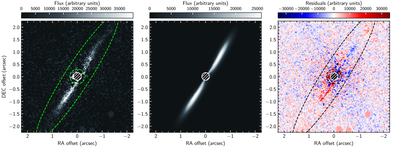
Fig. 3. Observation and model images for GSC 07396-00759. Shown from left to right are the measured Q_\phi , best-fit model and residual image obtained from our disk model using a linear scaling for each panel. The regions outside of the ellipse and within the circle (green dashed lines) are excluded from the \chi^2 calculation. The coronagraphic mask is indicated by the (shaded) circular region in each panel. North is to the top and east to left in each panel.
