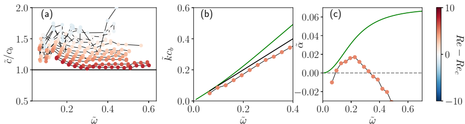
Figure 7: For carbopol ( n = 0.54 ), variation with the pulsation \bar{\omega} of (a) the normalised experimental phase speed \bar{c}/c_b , at different Re , (b) the wave number \bar{k} times c_b (dispersion relation), (c) the growth rate \bar{\alpha} . (b) and (c) correspond to the same case as in figure 4(a) ( Re = 11.2 , Bi = 0.29 ). Balmforth & Liu (2004) prediction: green line, for long waves: black line, experimental results: colored circles.
