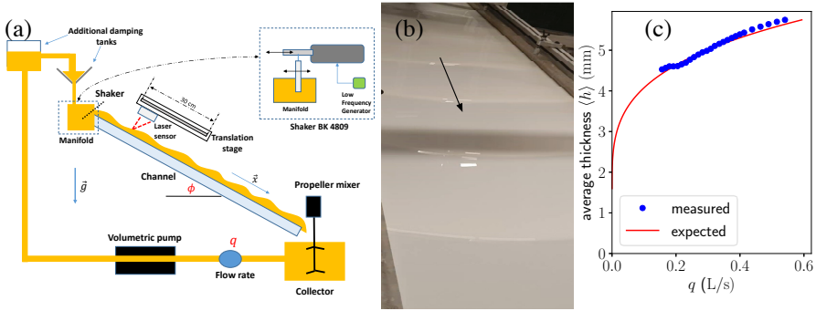
Figure 1: (a) Scheme of the experimental setup. (b) View of the experiment with unstable roll waves. Horizontal shadow is due to the measuring apparatus. (c) Average flow thickness: Values measured (sensor) and curve expected from flow rate and measured rheology, with a uniform flow hypothesis.
