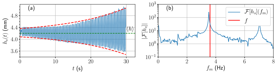
Figure 3: (a) Blue: typical measured signal h_s(t) . Red: signal envelope h_0 e^{\alpha vt} , with \alpha given by Eq. (2.3). (b) Blue: Fourier transform of signal h_s(t) . Red: imposed frequency at 3.6 Hz. The main peak is at a frequency \Re(f^*) = f - kv/2\pi , slightly shifted from the imposed frequency.
