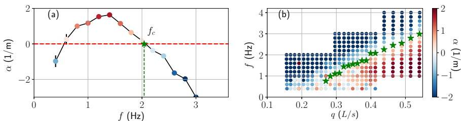
Figure 4: (a) Variation of the growth rate \alpha with the frequency f , at flow rate q = 0.412 \text{ dm}^3 \cdot \text{s}^{-1} and at angle \phi = 15.6^\circ , for carbopol with a rheology \tau_y = 4.21 \text{ Pa} , K = 0.99 \text{ Pa} \cdot \text{s}^n , n = 0.54 . (b) Stability map in the (q, f) plane (same \phi and rheology as in (a)). Green stars: cutoff frequencies. In both pictures, colors correspond to growth rate \alpha (see the scale in (b)).
